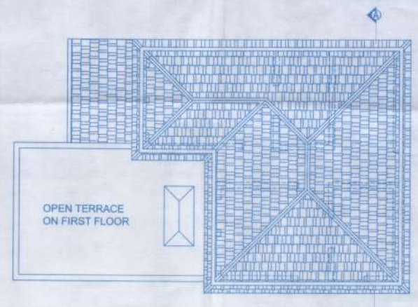
ROOF PLAN 1:100
