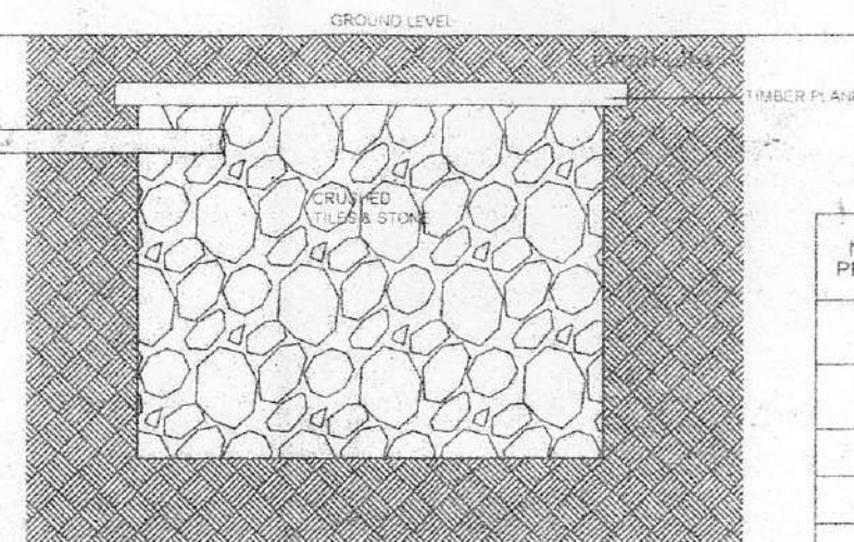
CROSS-SEC. SOAK PIT
