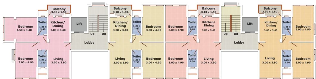
TYPICAL FIRST, SECOND, THIRD, FOURTH FLOOR PLAN
