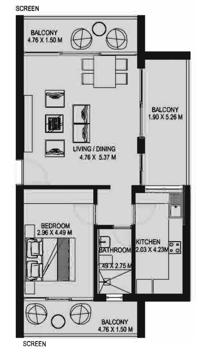
1BHK CANTILEVER APARTMENT
