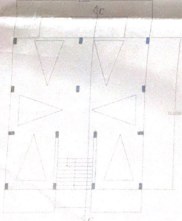
STILT FLOOR PLAN SC. 1:100
