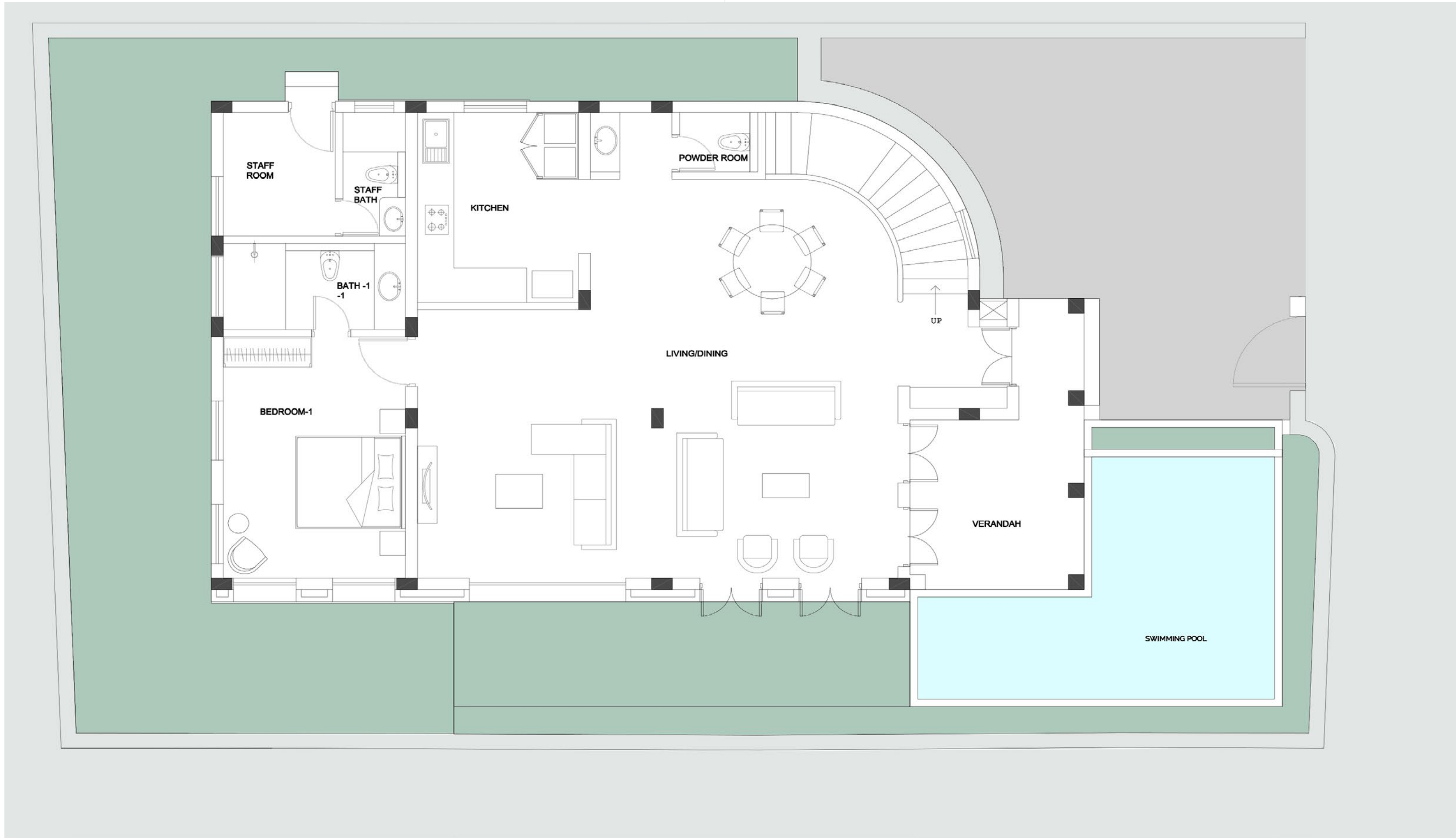
VILLA "A" GROUND FLOOR
