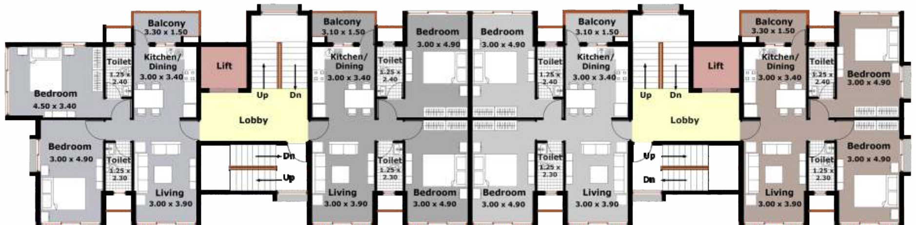
Typical 1st to 4th Floor plan
