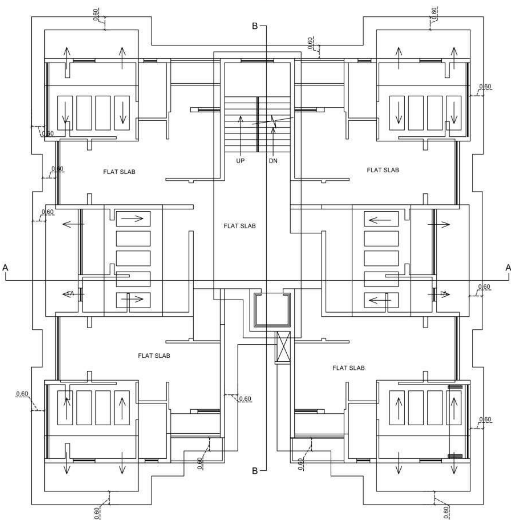
ROOF FLOOR PLAN
