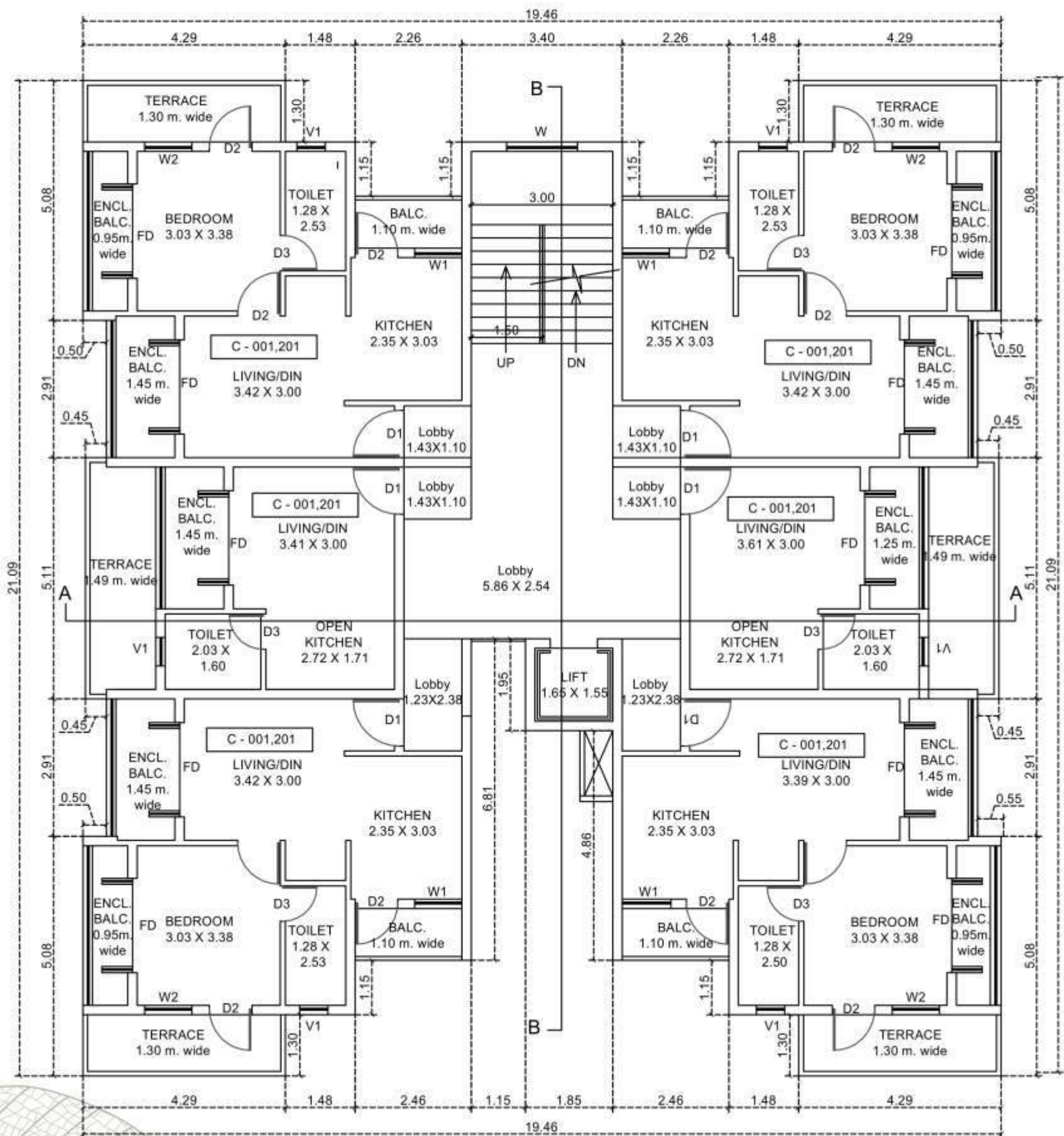
TYPICAL UPPER GROUND FLOOR PLAN
