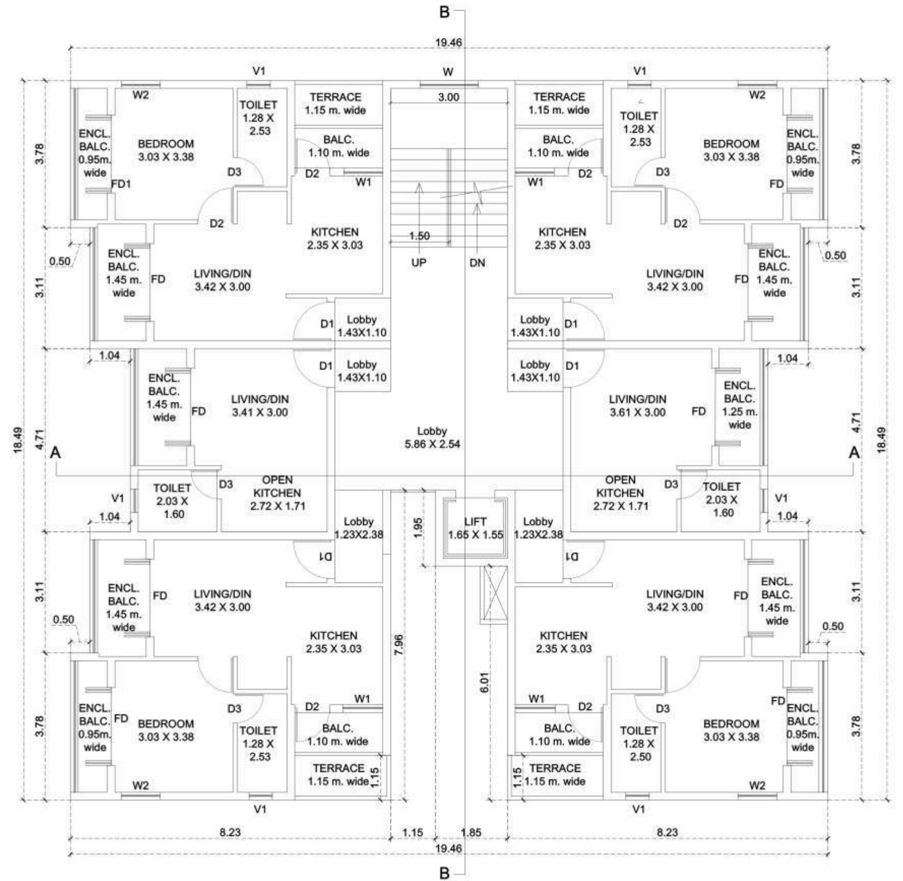
TYPICAL FIRST AND THIRD FLOOR PLAN
