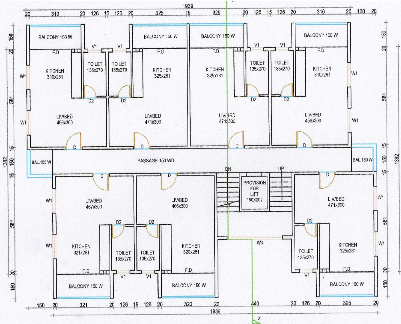
TYPICAL FIRST & SECOND FLOOR PLAN BLOCK-A SCALE-1:100
