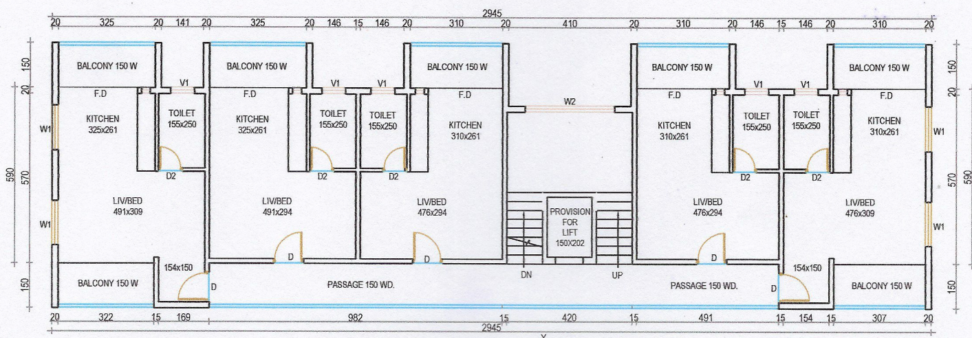
TYPICAL FIRST & SECOND FLOOR PLAN BLOCK-B SCALE-1:100
