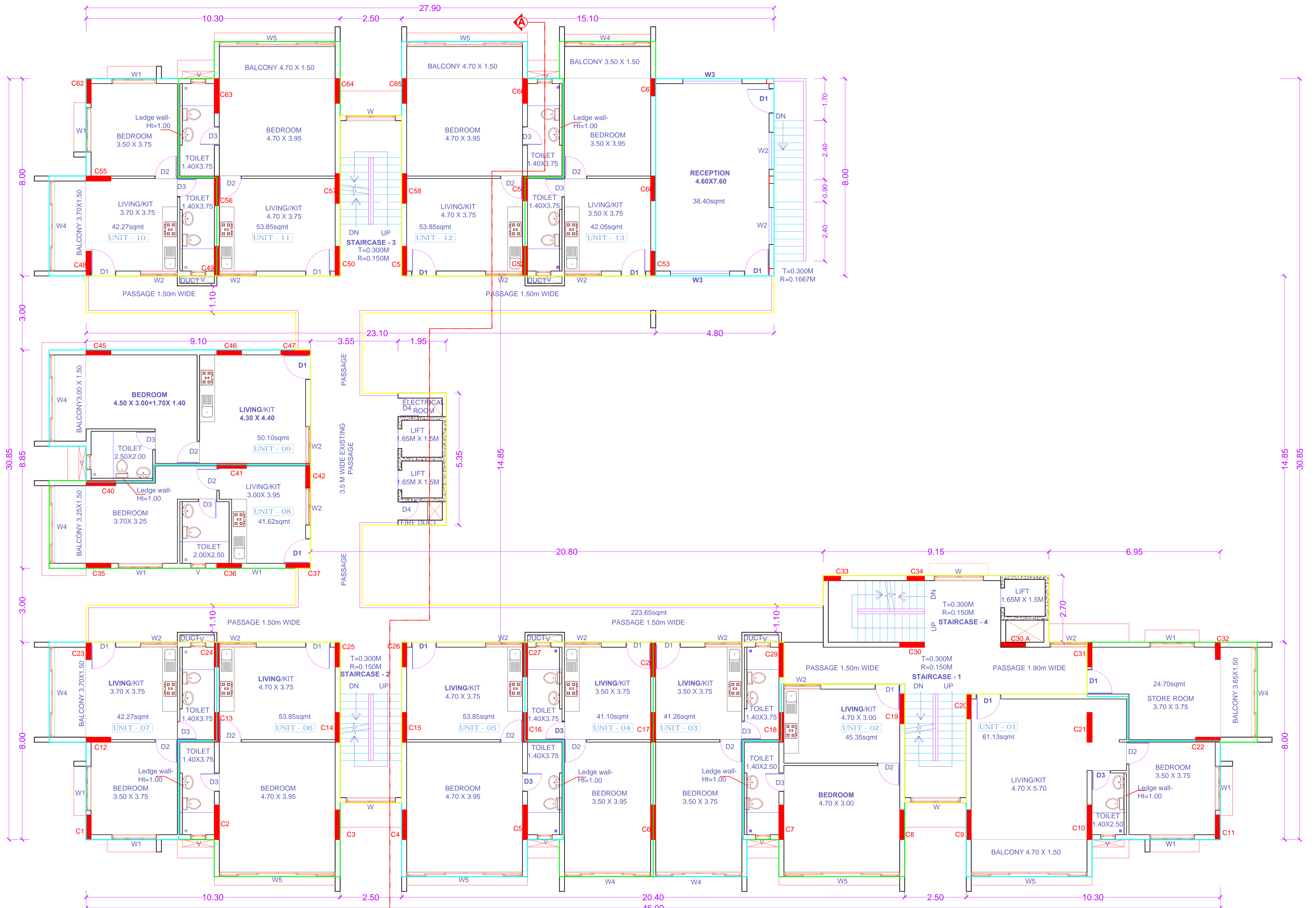
FIRST FLOOR PLAN SCALE 1:100
