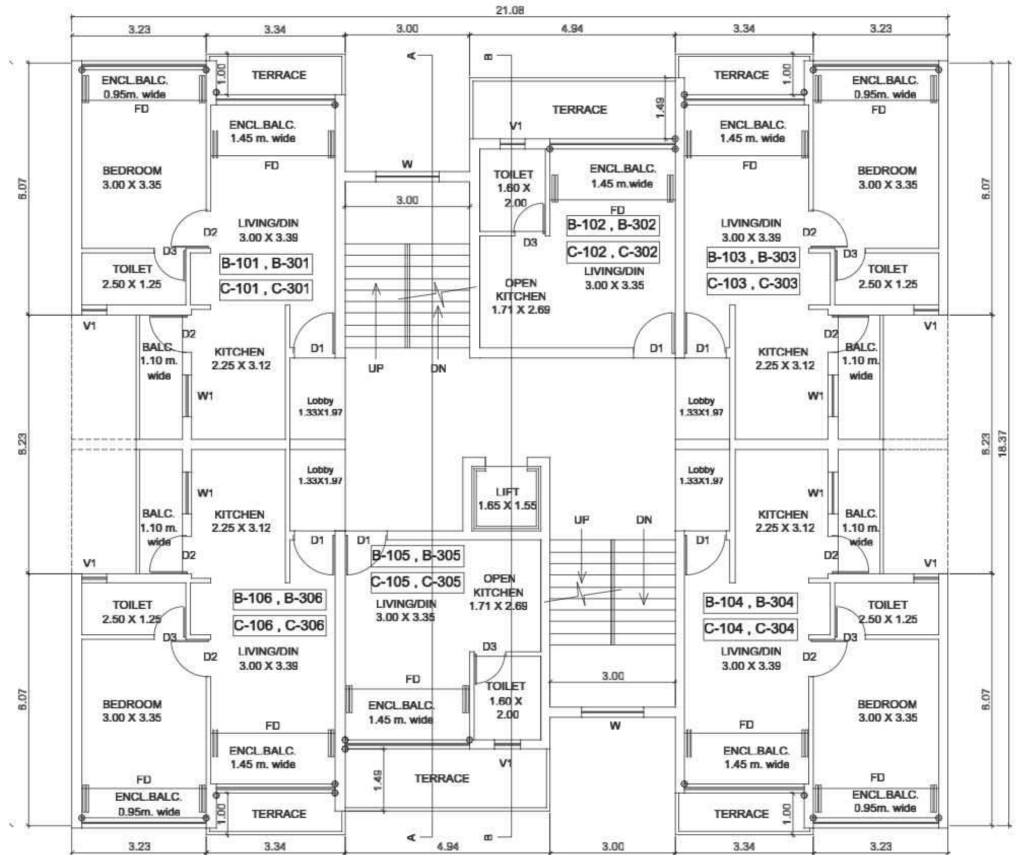
TYPICAL FIRST & THIRD FLOOR PLAN
