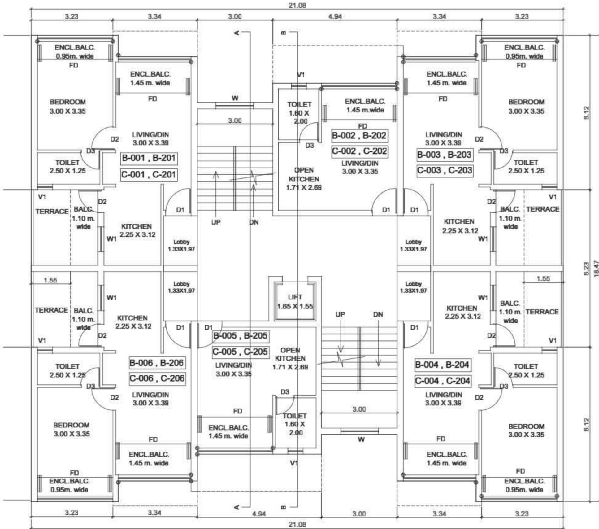
TYPICAL UG, SECOND & FOURTH FLOOR PLAN
