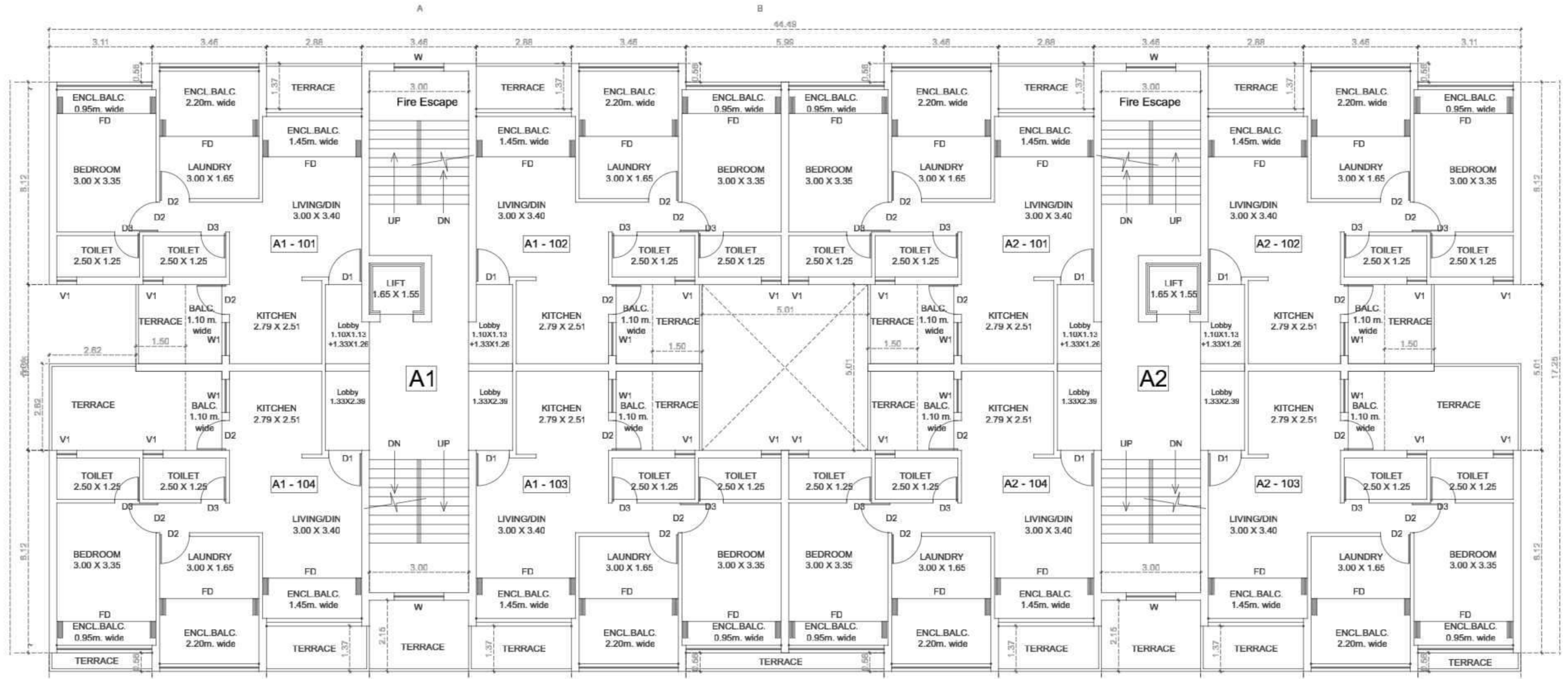
TYPICAL FIRST & THIRD FLOOR PLAN
