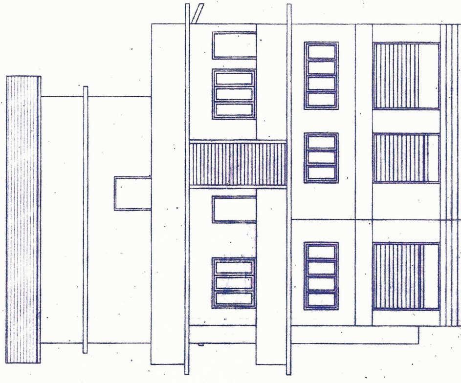
FRONT ELEVATION (1:100)
