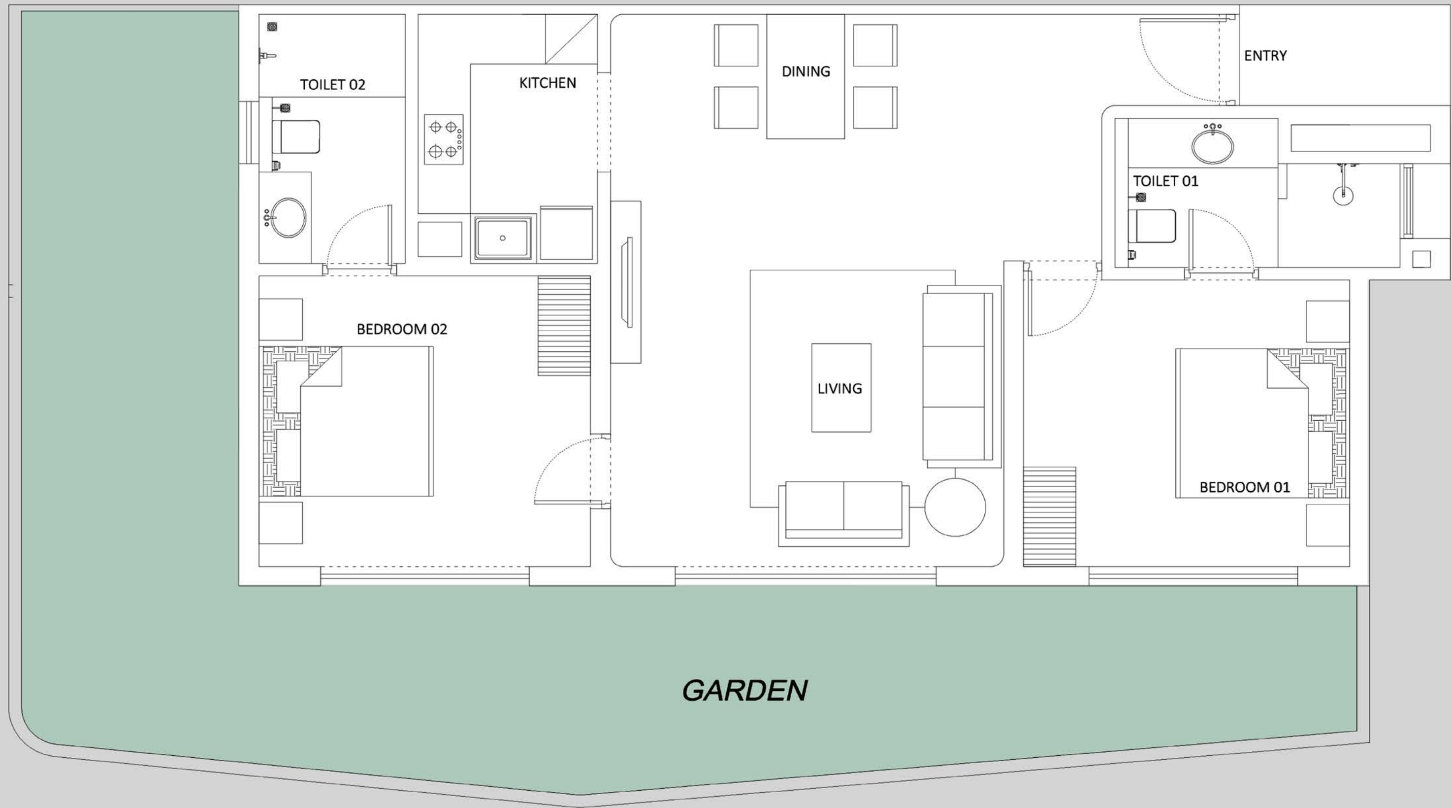
GROUND FLOOR
