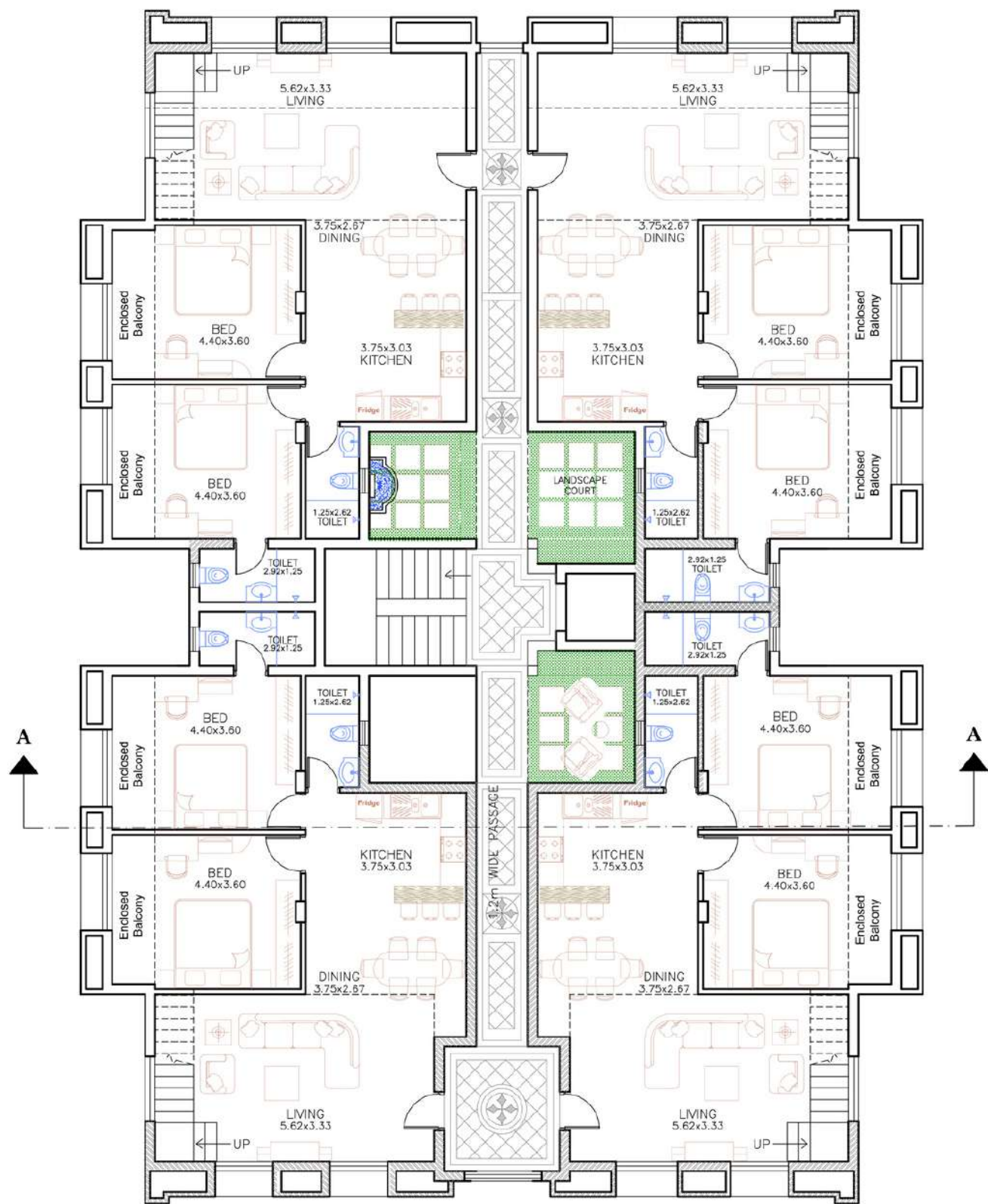
FIRST FLOOR
