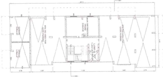
LOWER GROUND FLOOR PLAN scale 1:100
