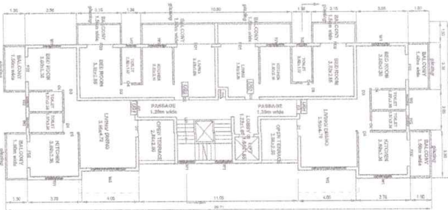
UPPER GROUND FLOOR PLAN scale 1:100
