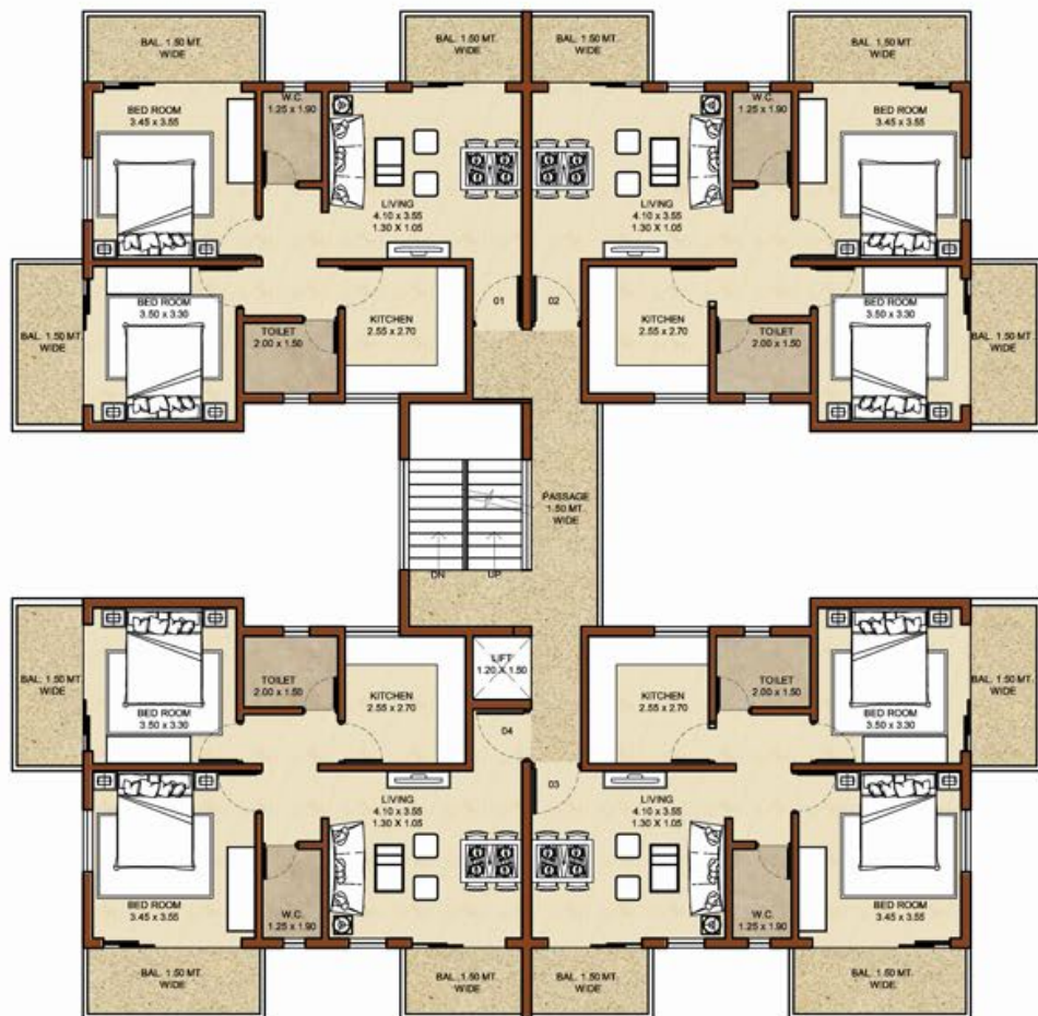
TYPICAL FLOOR PLAN BLOCK B
