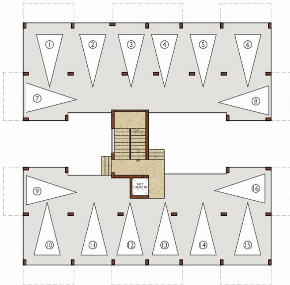
STILT LEVEL PLAN BLOCK B
