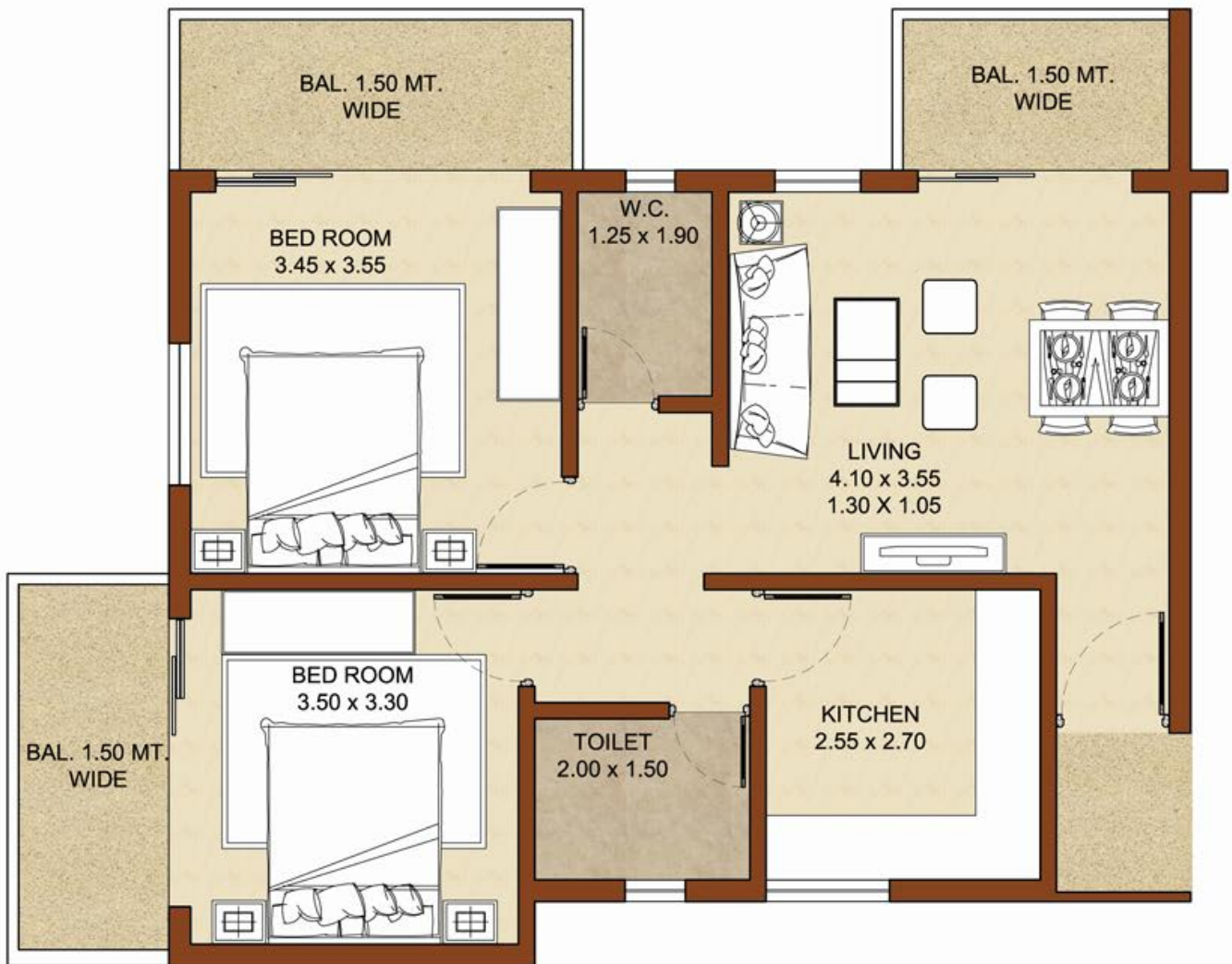
UNIT PLAN BLOCK B- APARTMENT 01
