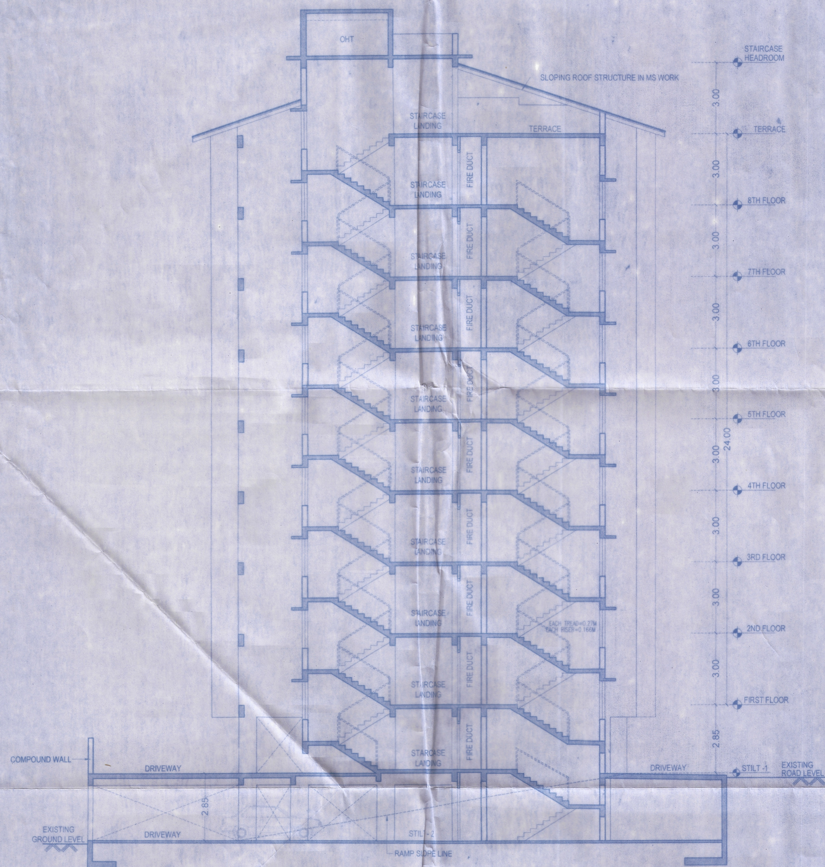
SECTION-AA SCALE-1:100
