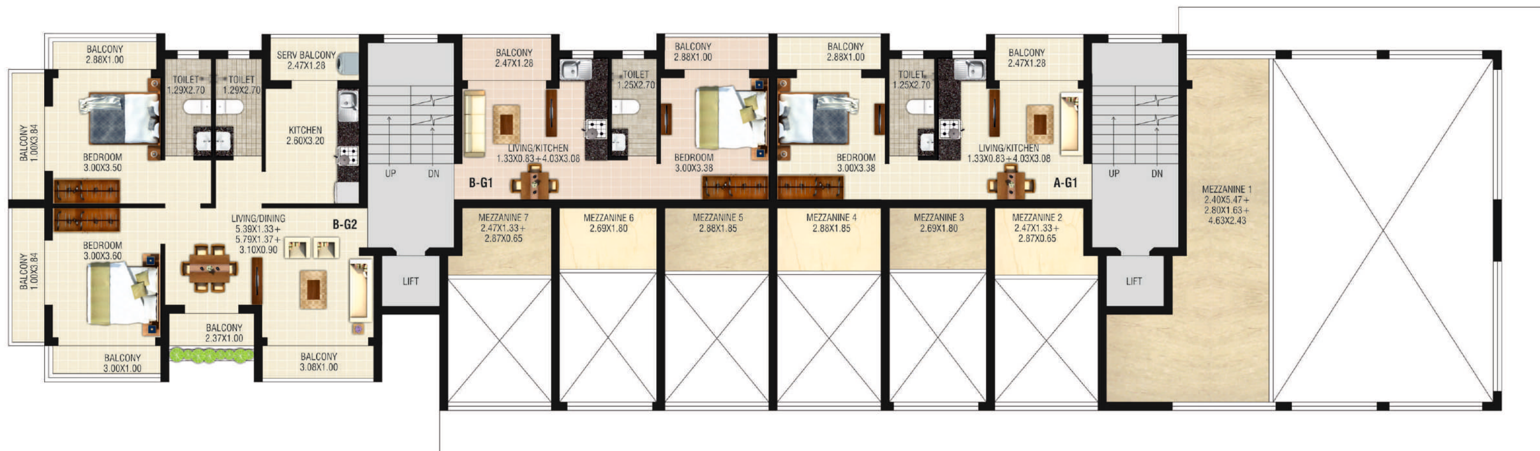
UPPER GROUND FLOOR PLAN
