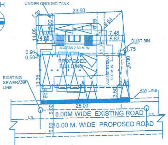
PARKING LAYOUT PLAN (SCALE 1:500)
