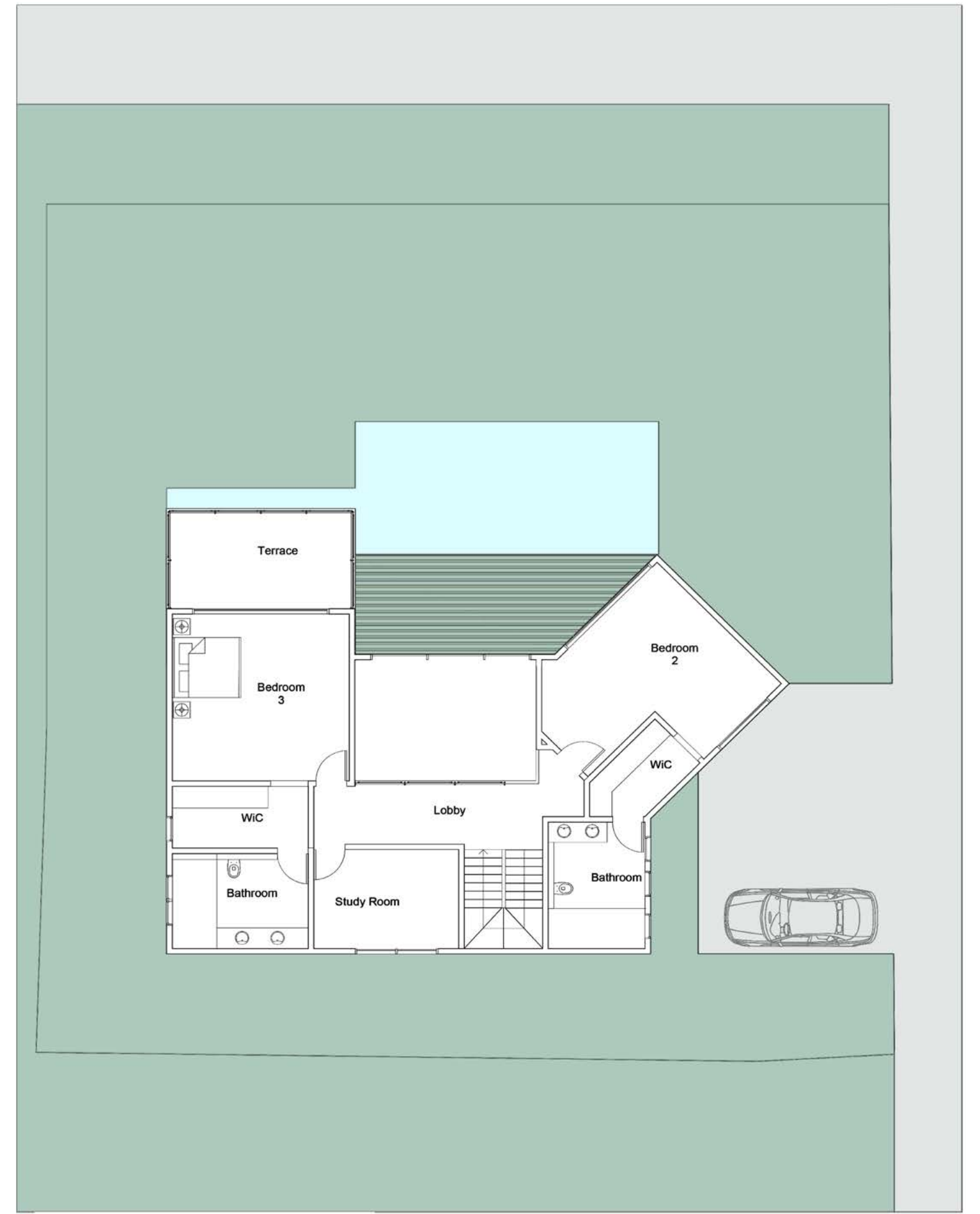
FIRST FLOOR
