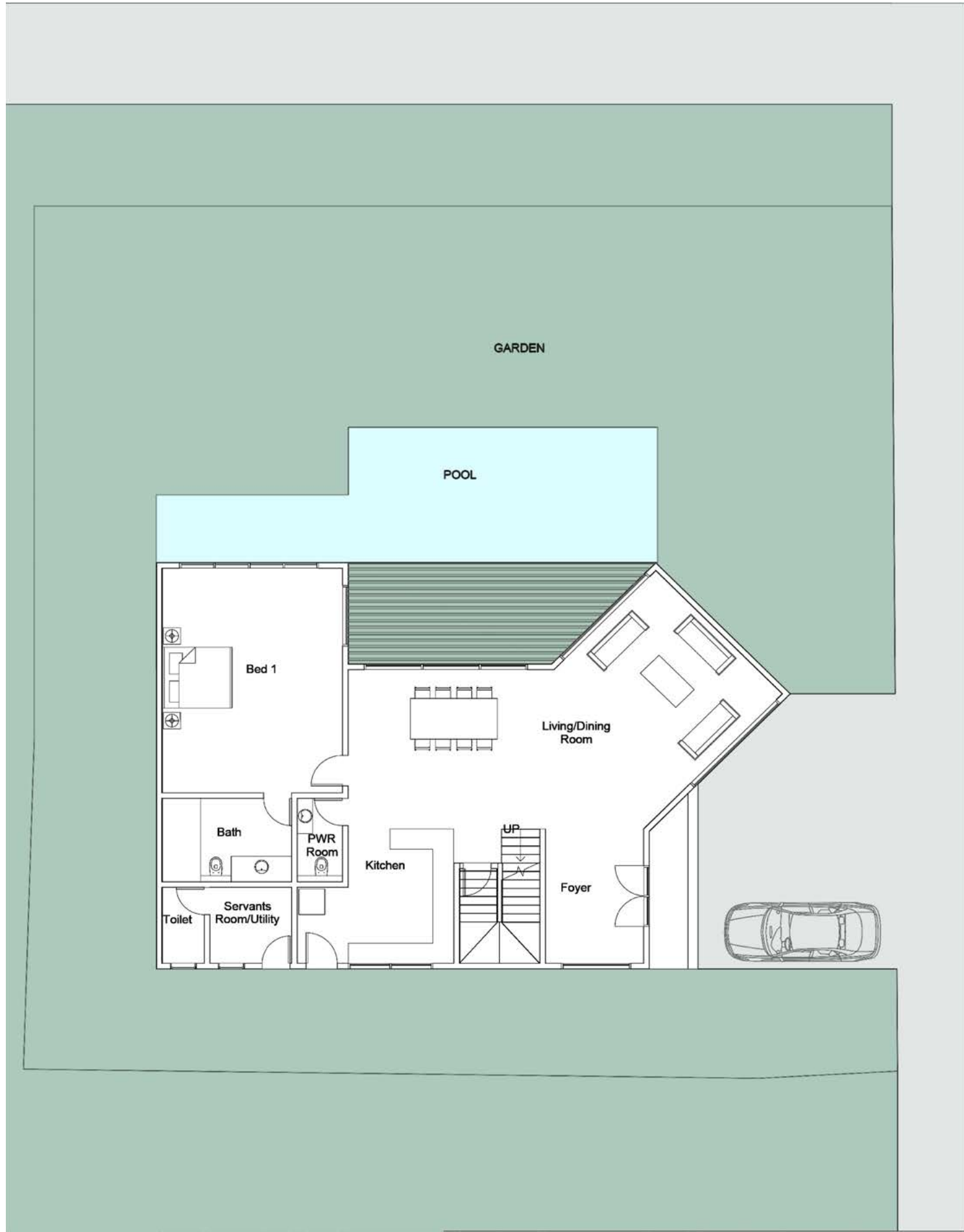
GROUND FLOOR
