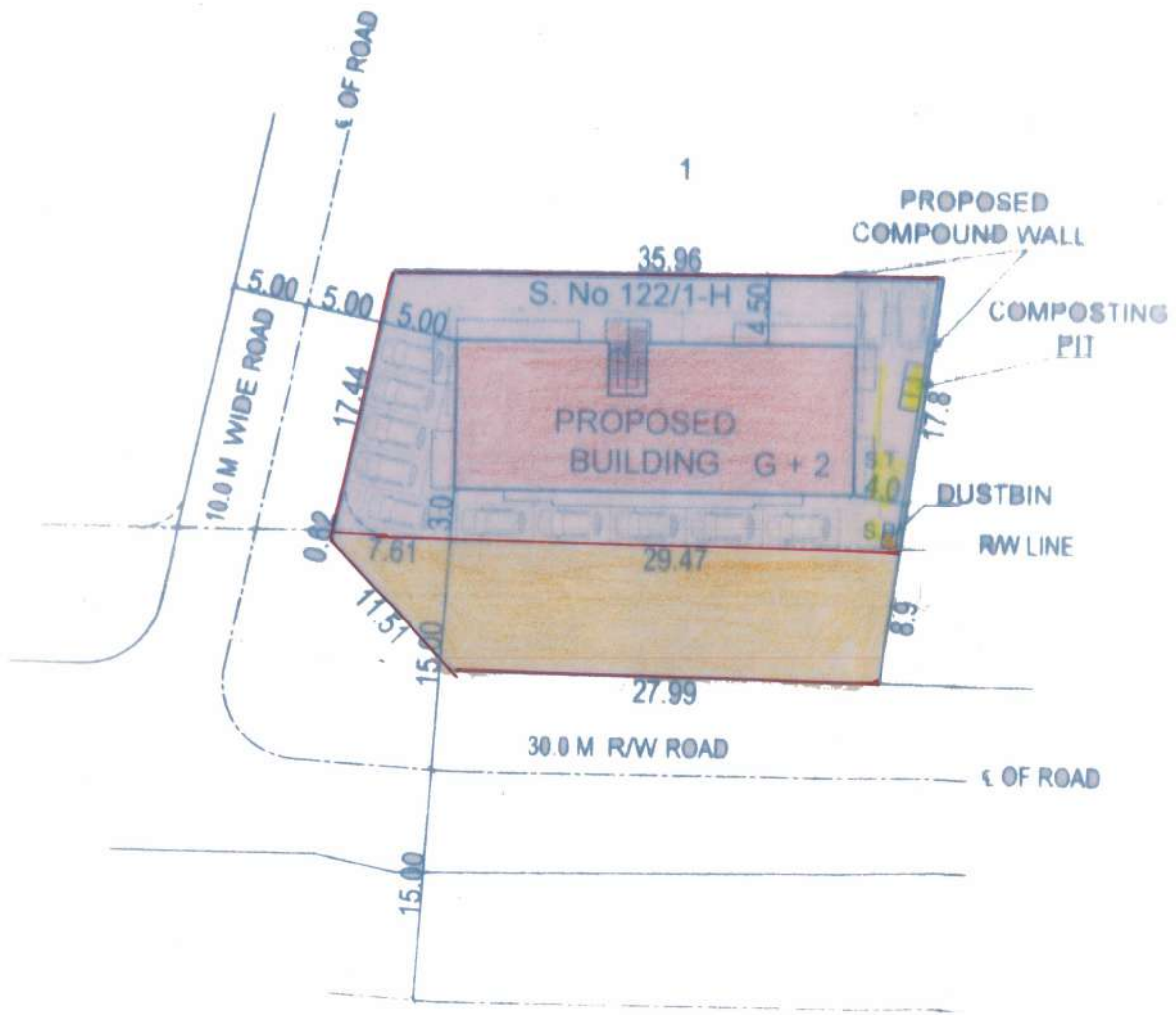
SITE PLAN
