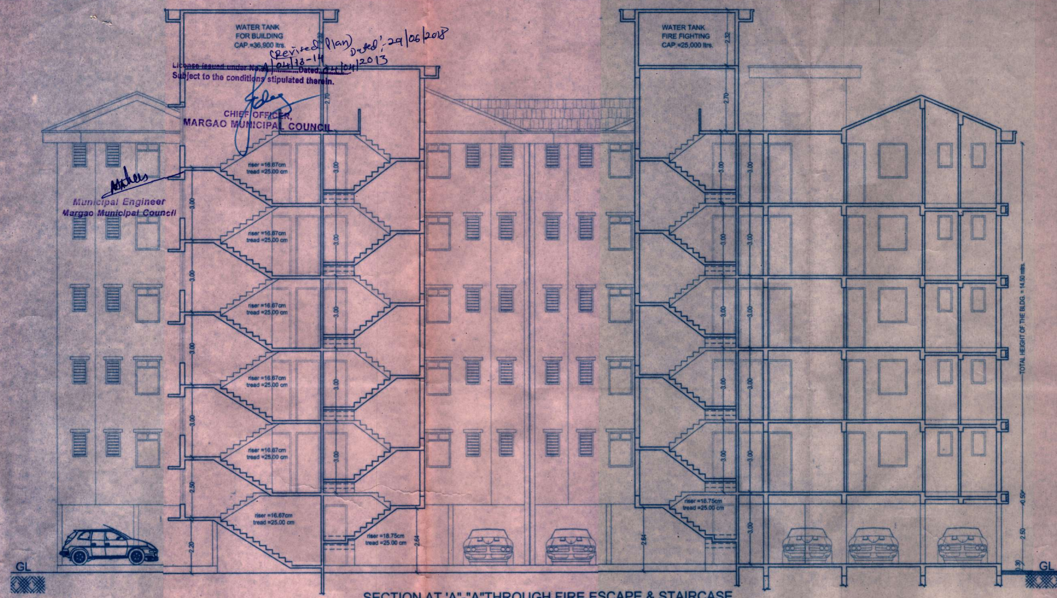
SECTION AT 'A'- 'A' THROUGH FIRE ESCAPE & STAIRCASE
