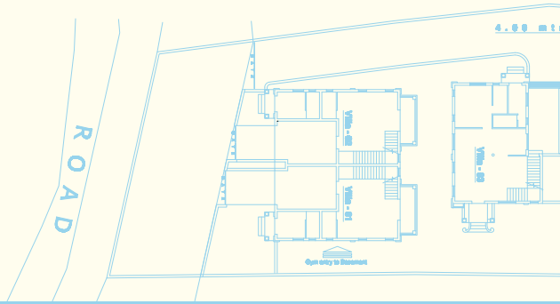
First Floor Plan : Villa 5 & 6
