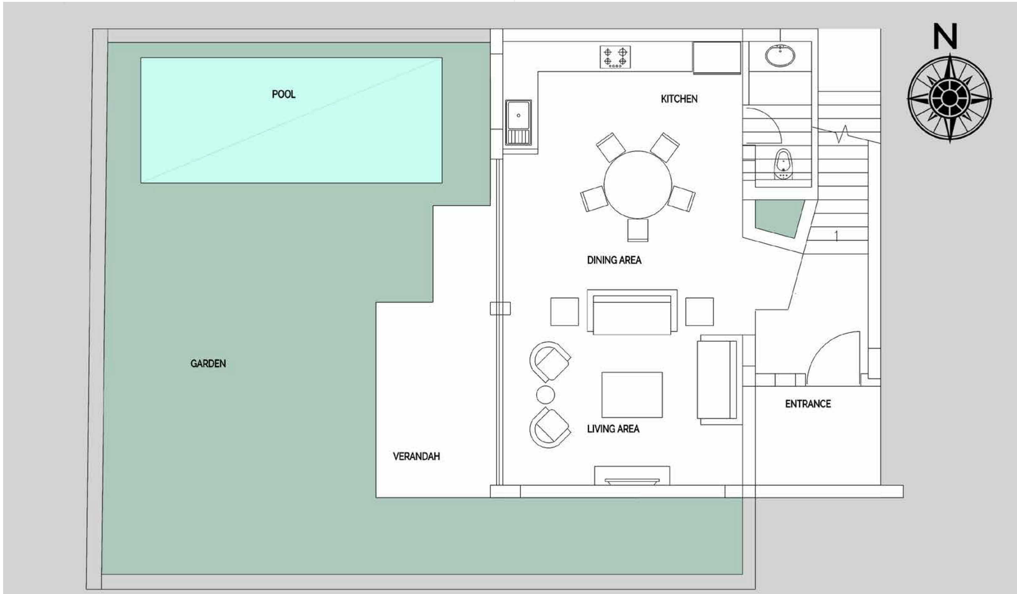
GROUND FLOOR
