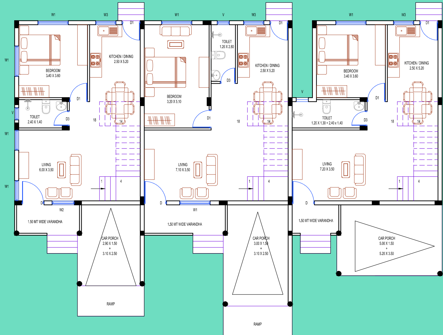
GROUND FLOOR ( PROPOSED VILLA C,D,E )
