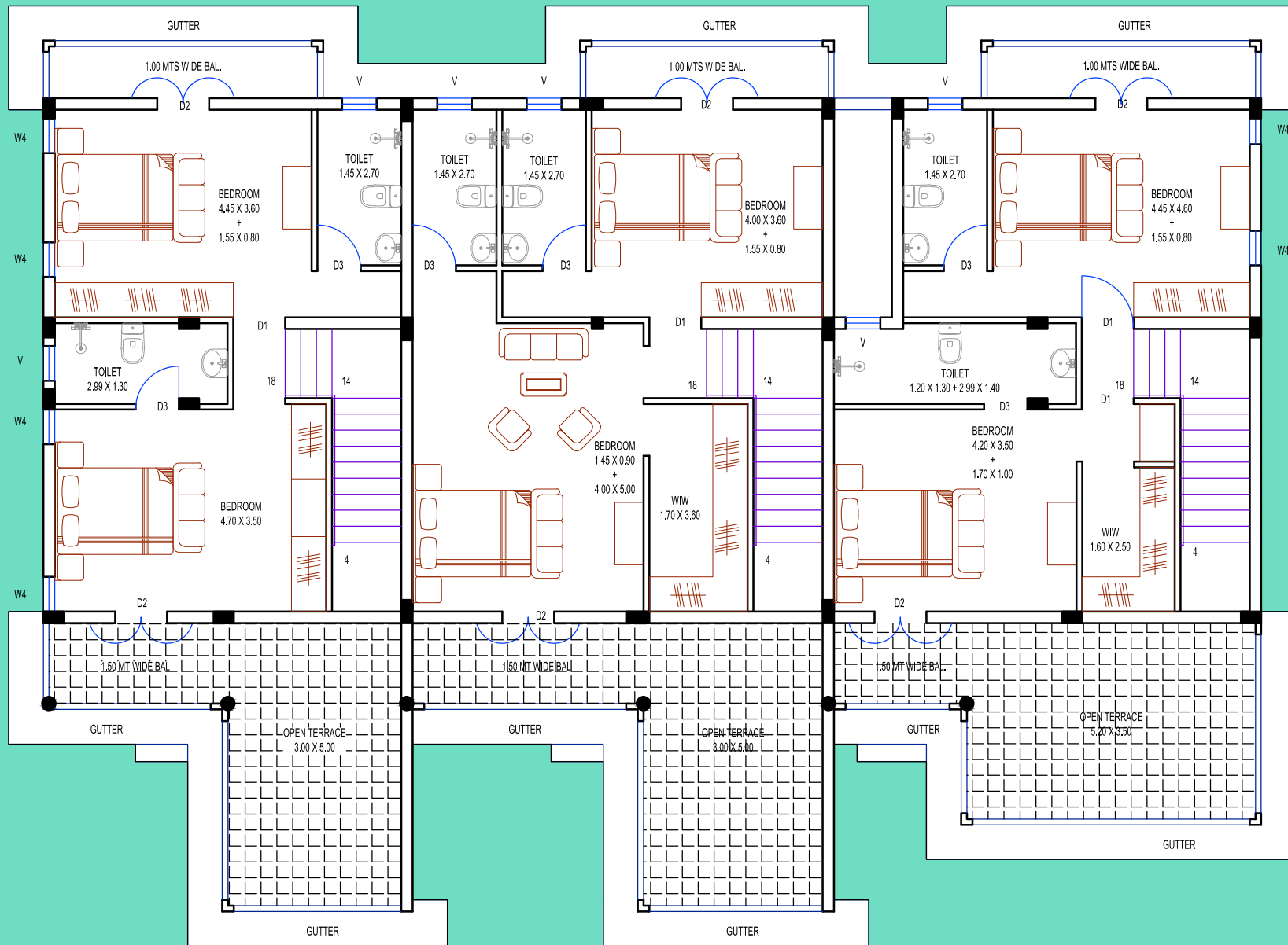
FIRST FLOOR ( PROPOSED VILLA C,D,E )
