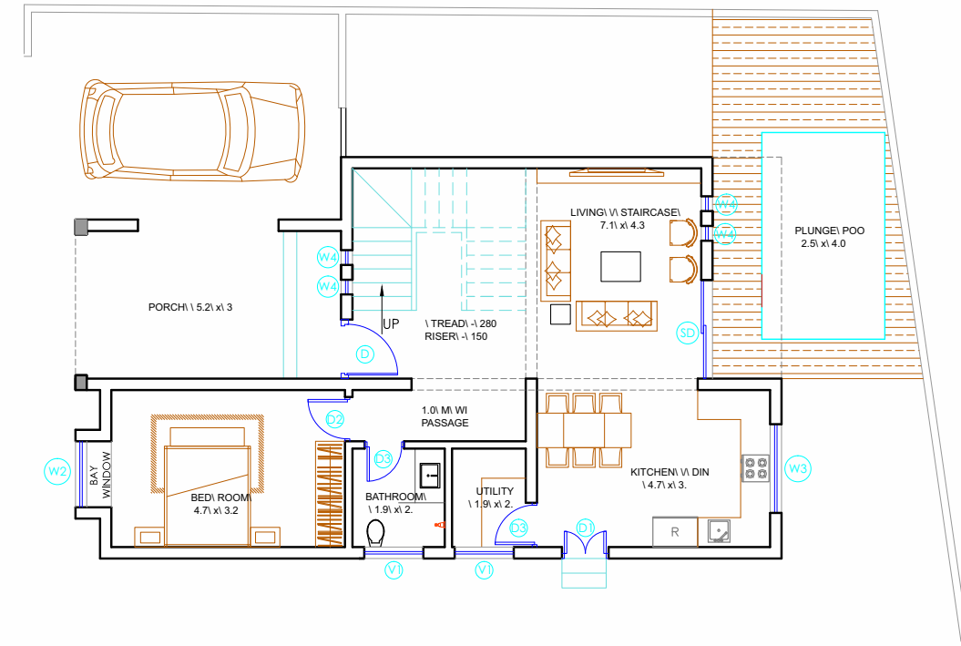
GROUND FLOOR LAYOUT SCALE 1:10
