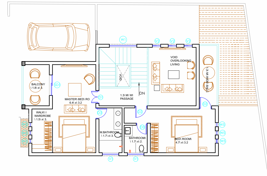
FIRST FLOOR LAYOUT SCALE 1:10
