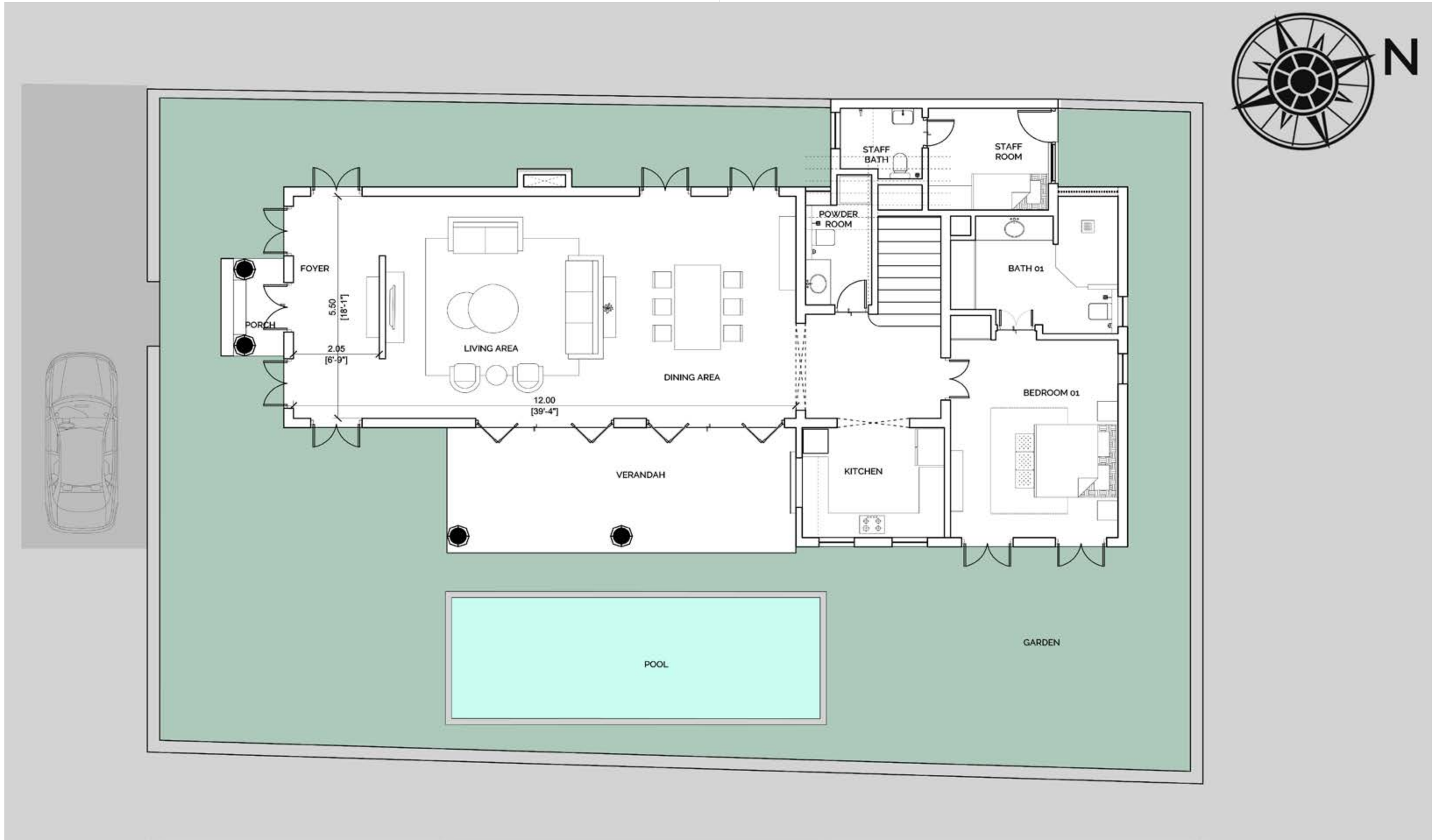
TYPE C GROUND FLOOR
