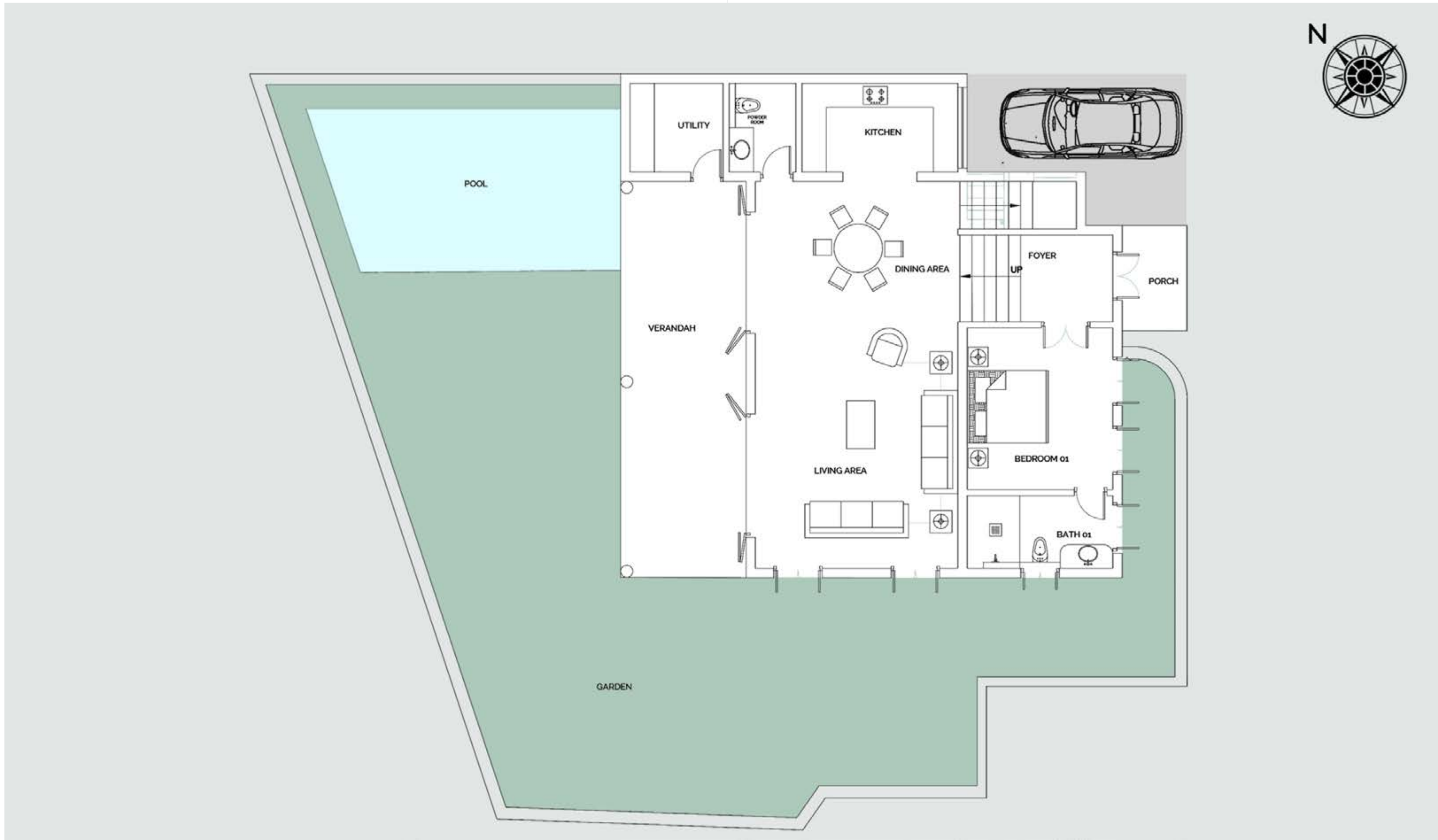
TYPE I GROUND FLOOR
