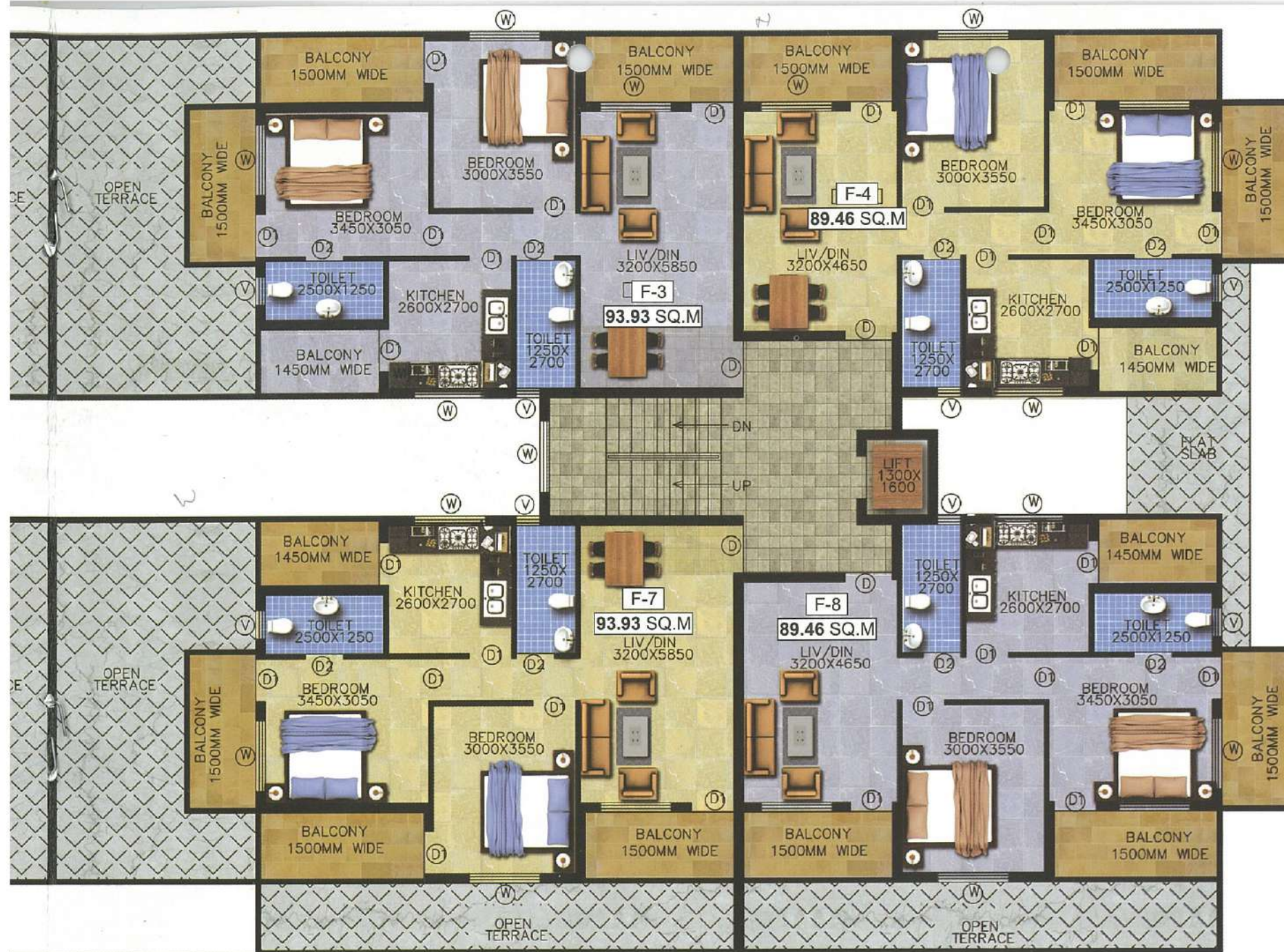
T FLOOR PLAN
