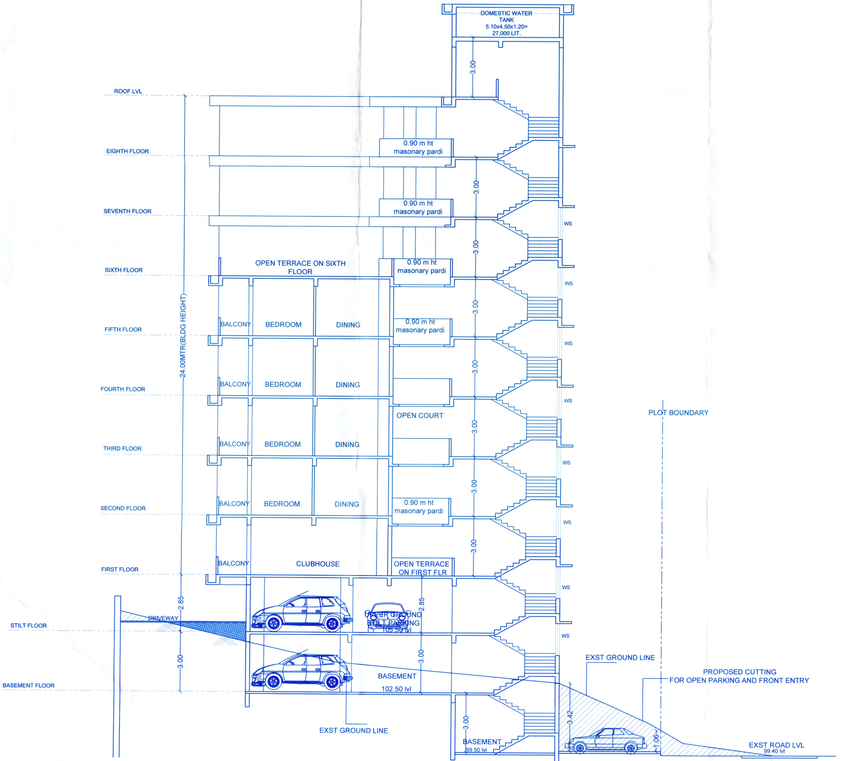
SECTION AA TREAD=30 CM RISER=16.66 CM
