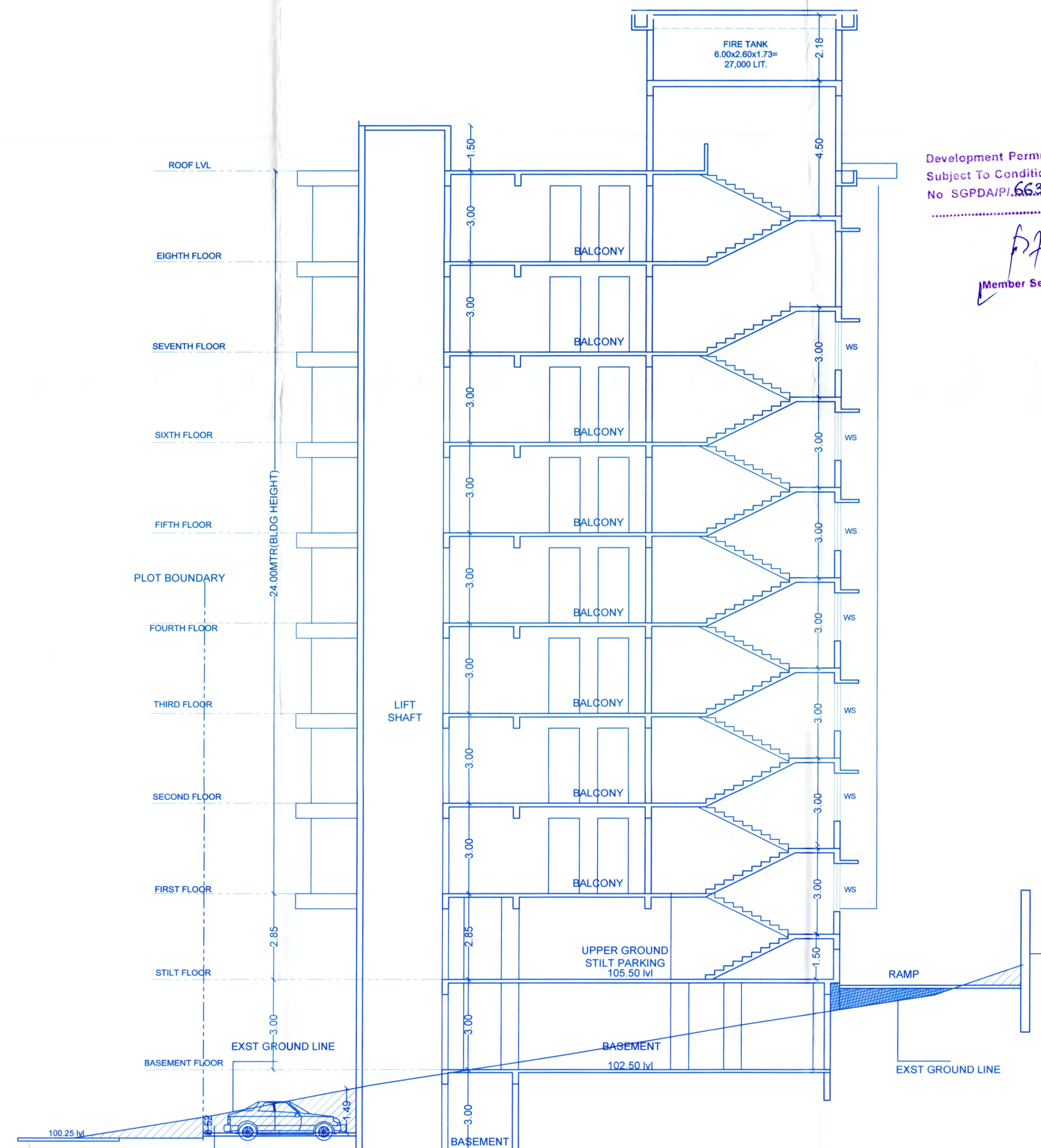
SECTION BB THROUGH FIRE STAIR TREAD=30 CM RISER=15.00 CM
