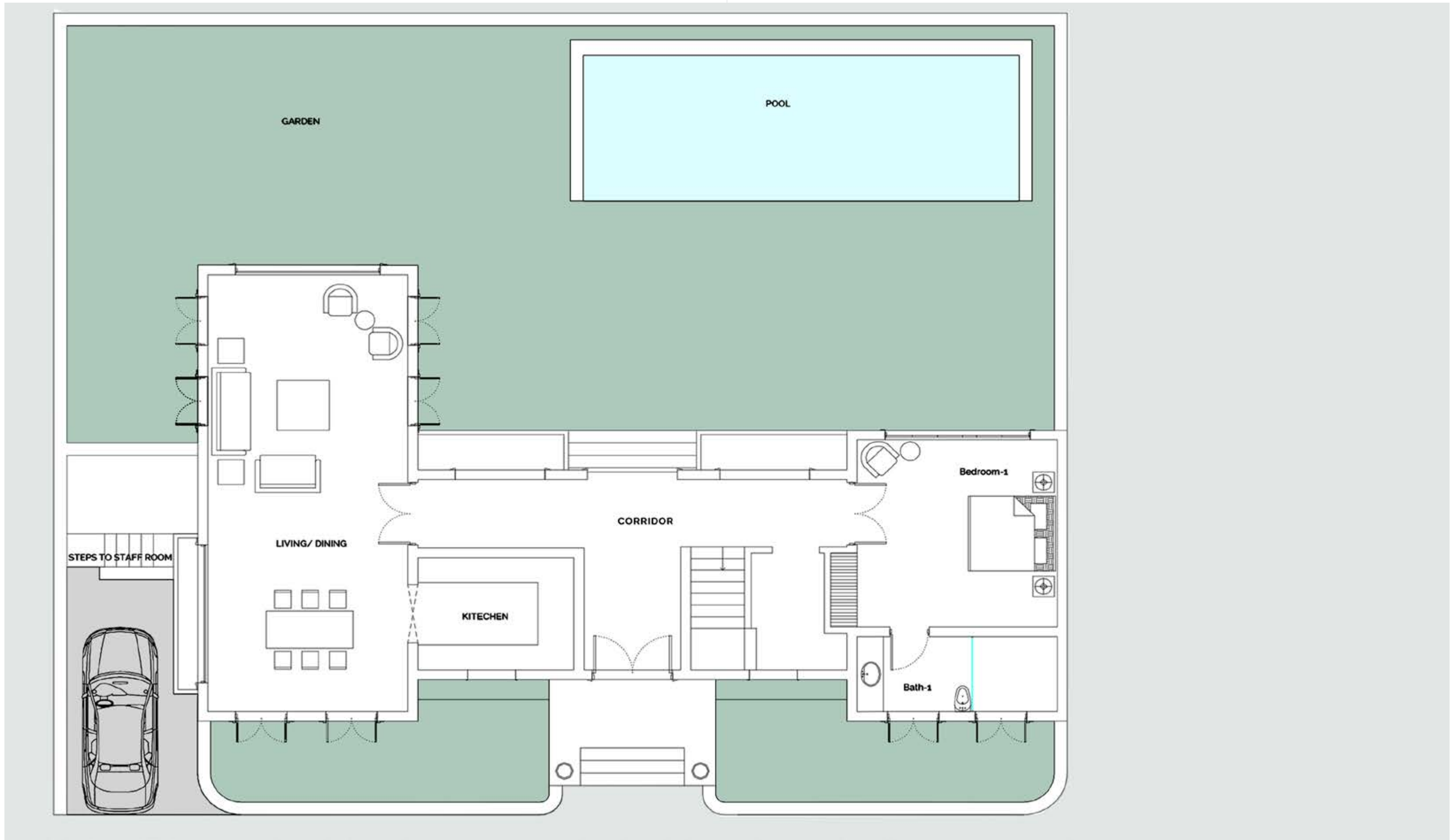
TYPE 1 GROUND FLOOR PLAN
