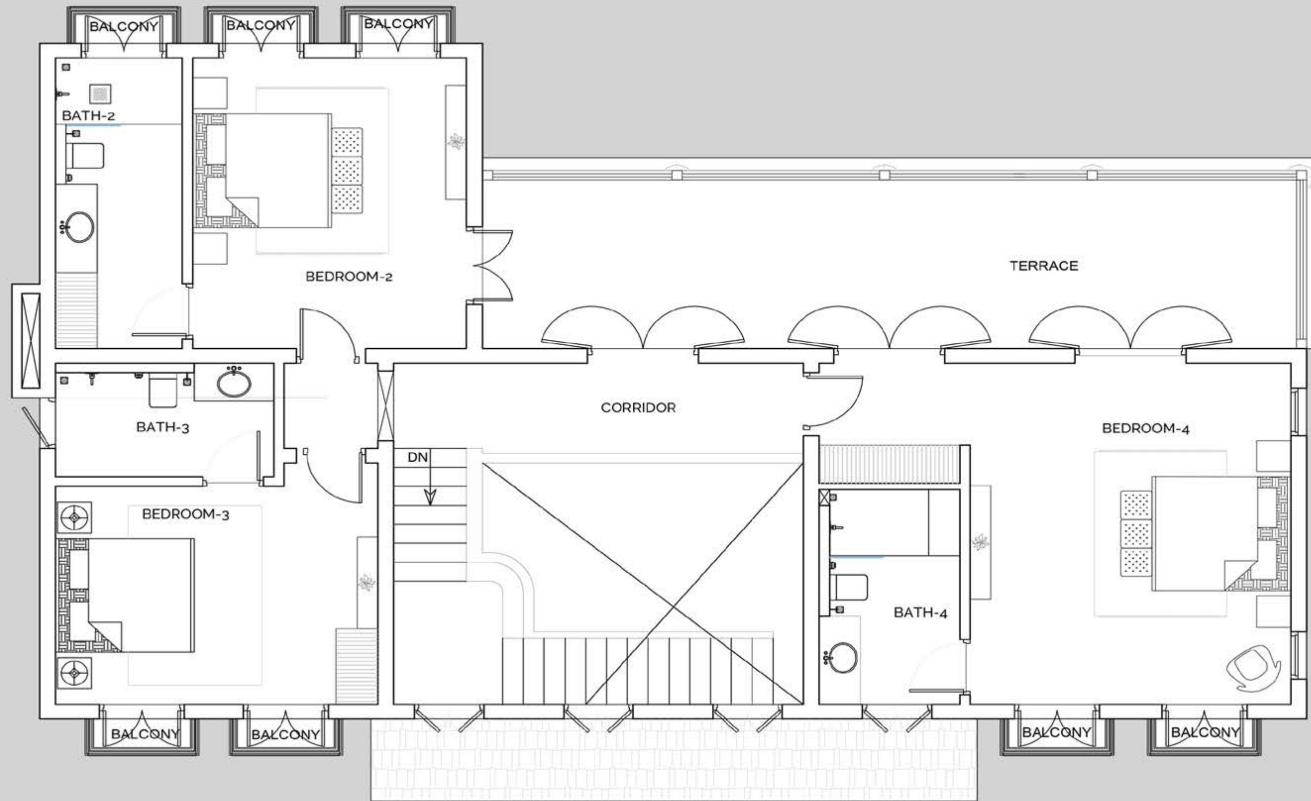
FIRST FLOOR
