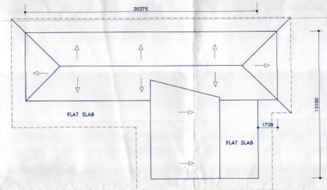
ROOF LAYOUT PLAN
