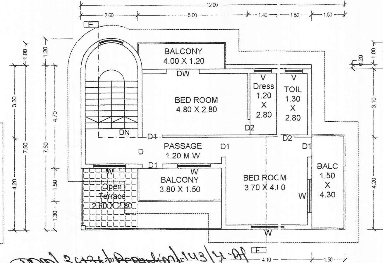
SECOND FLOOR PLAN SC 1:100 BUILT UP AREA 75.30 M2
