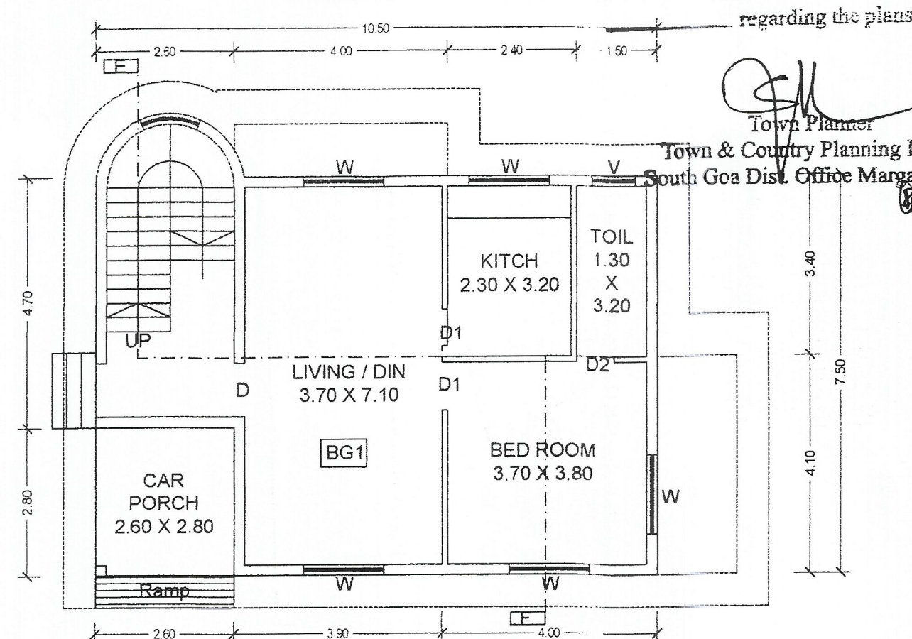
GROUND FLOOR PLAN SC 1:100 BUILT UP AREA OF BUNGALOW 78.75 M2
