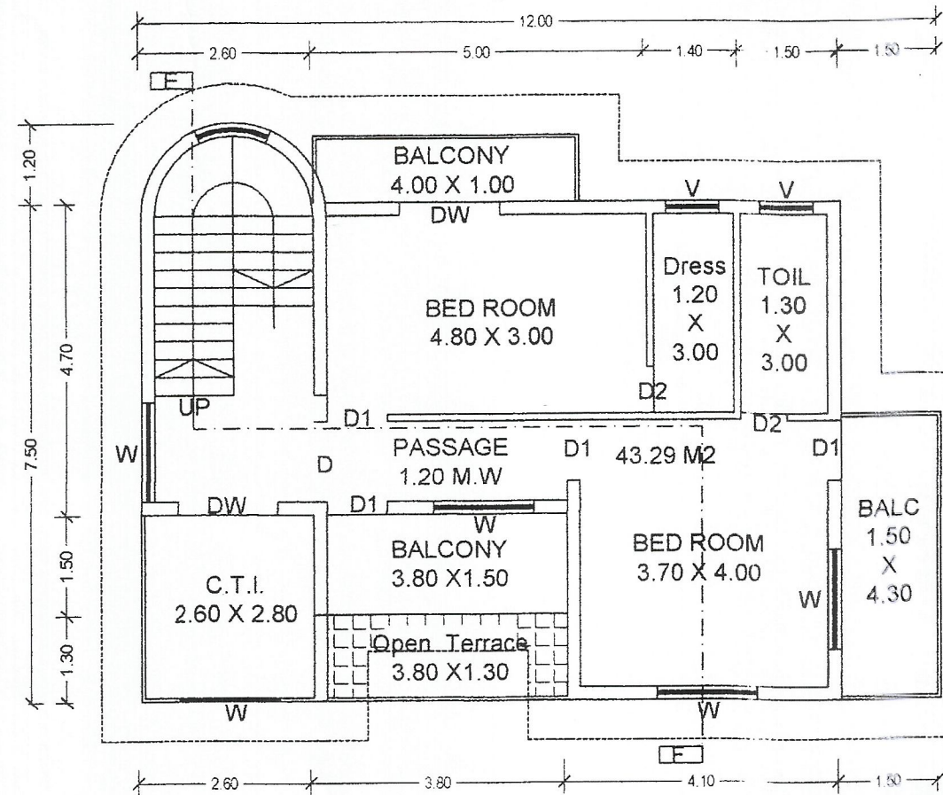
FIRST FLOOR PLAN SC 1:100 BUILT UP AREA 79.44 M2
