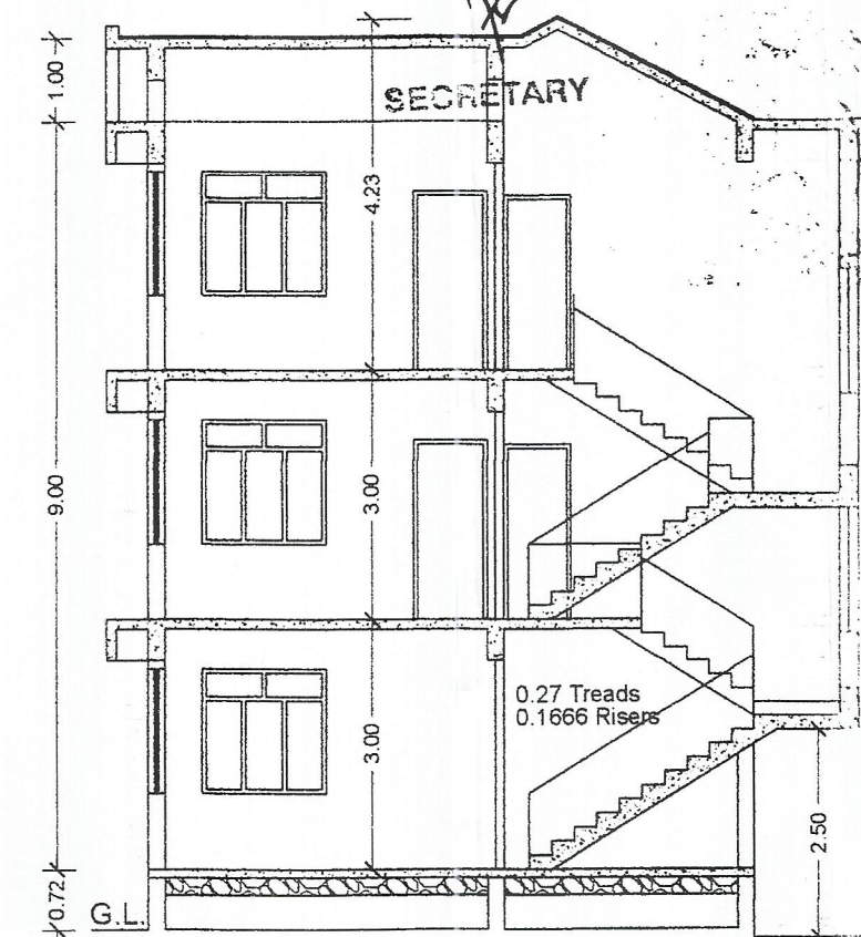
SECTION AT E-F SC 1:100
