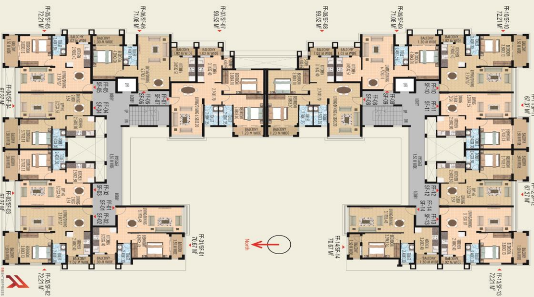
Typical First & Second Floor Plan
