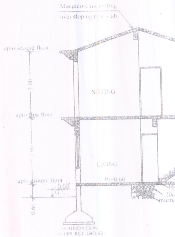
SECTION X-X
