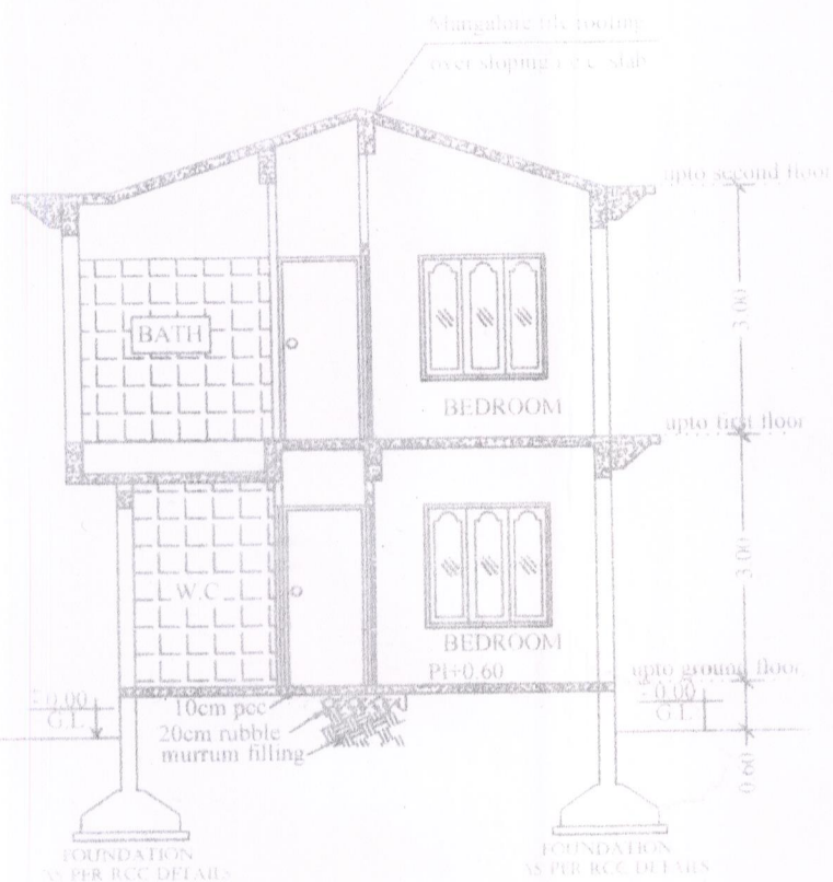
SECTION Y-Y
