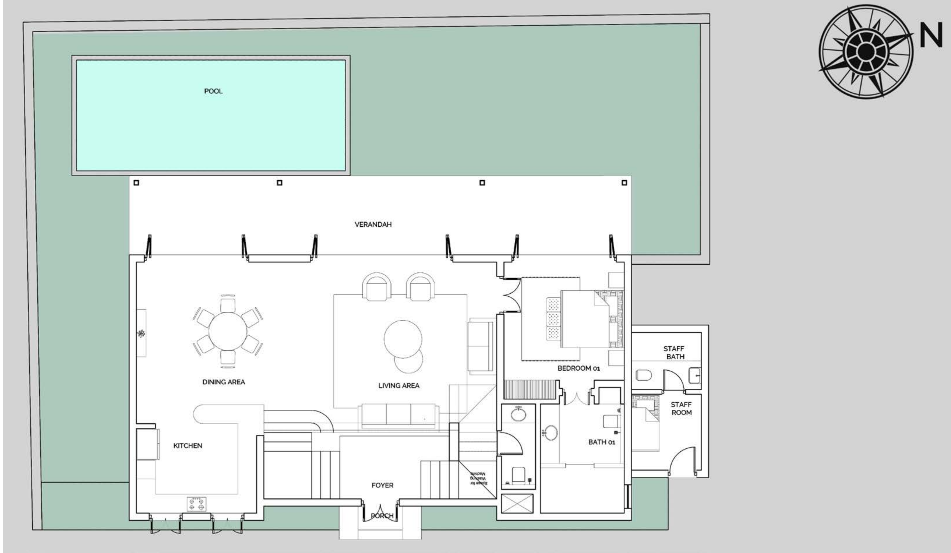
GROUND FLOOR
