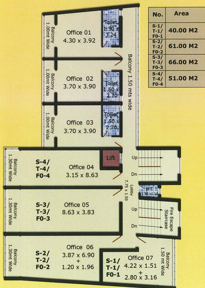
Second, Third & Fourth Floor Plan
