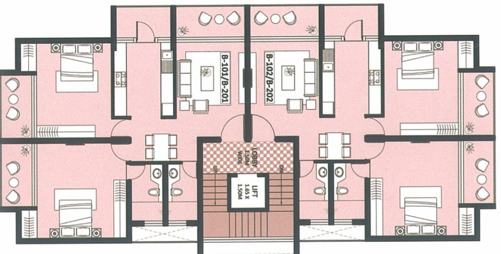
TYPICAL FIRST & SECOND FLOOR PLAN OF BLOCK B
