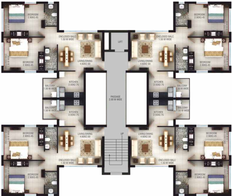
Upper Ground, First & Second Floor Plan
