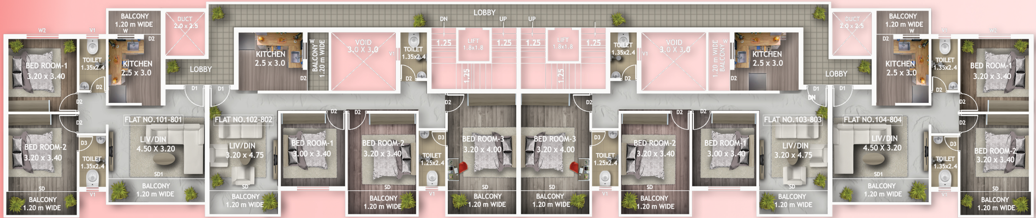
1ST FLOOR TO 8TH FLOOR PLAN SCALE - 1:100
