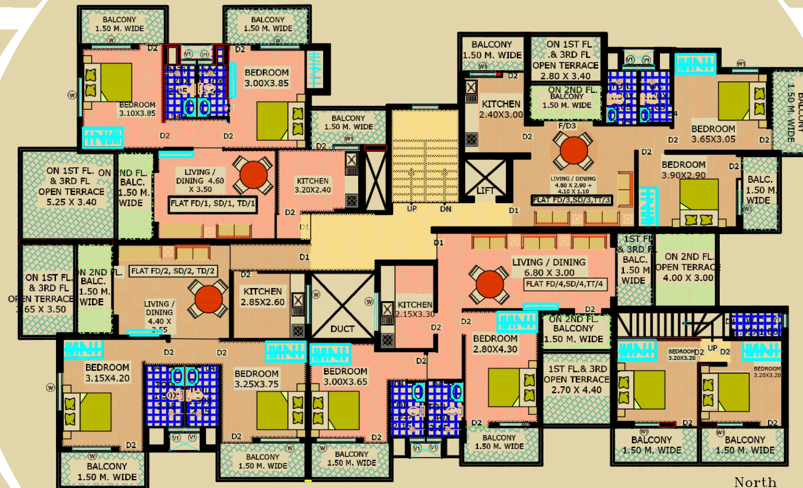
TYPICAL FIRST SECOND THIRD FLOOR PLAN
