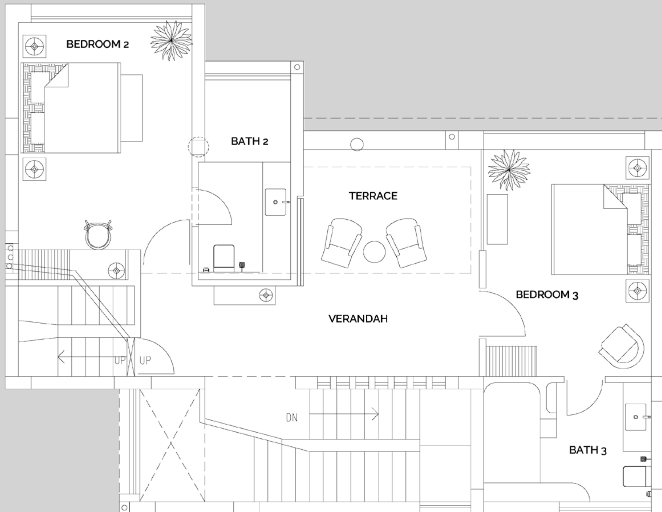
FIRST FLOOR TYPE O2
