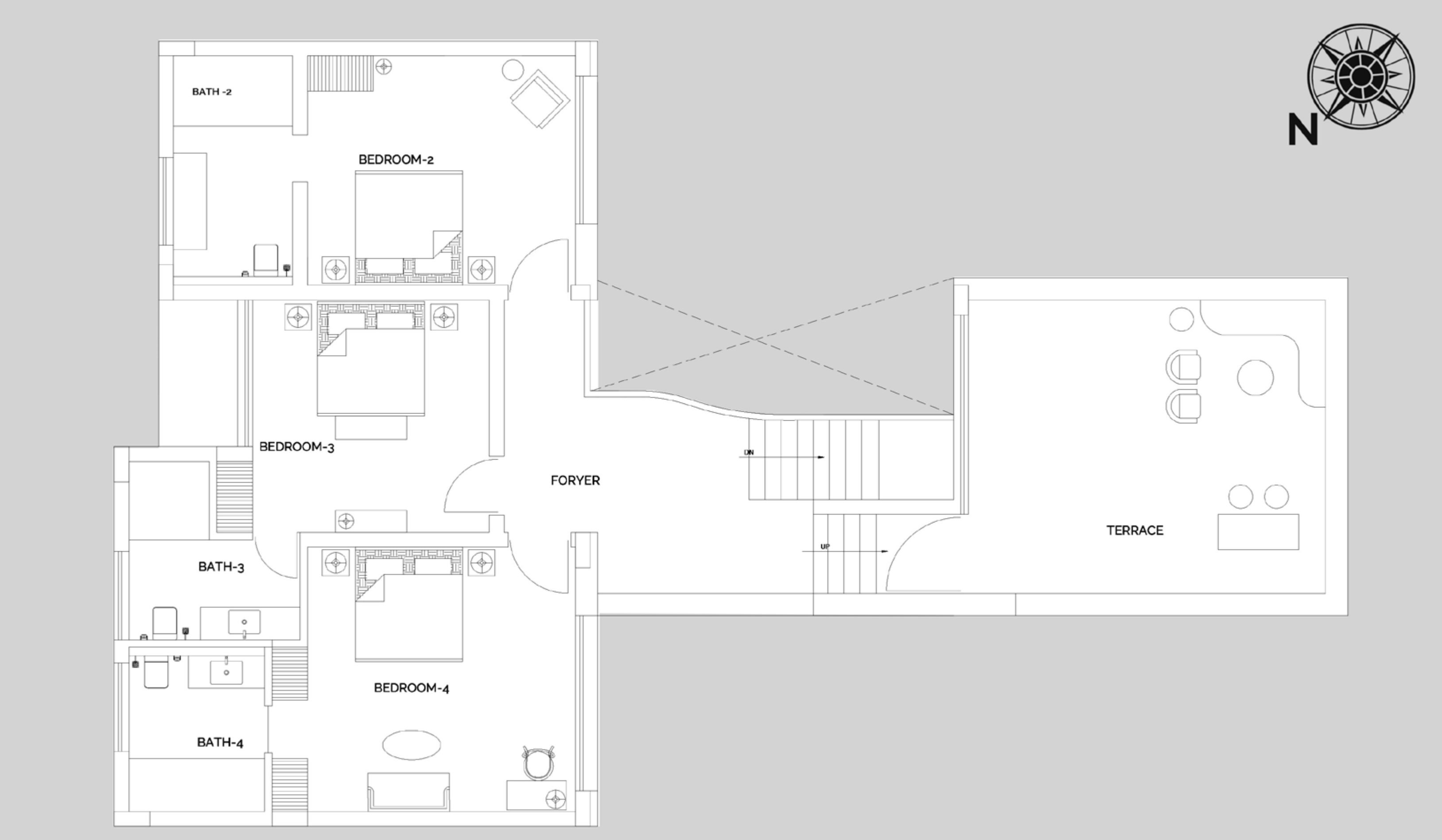
FIRST FLOOR TYPE01
