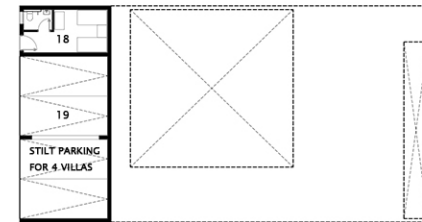
STILT FLOOR PLAN
