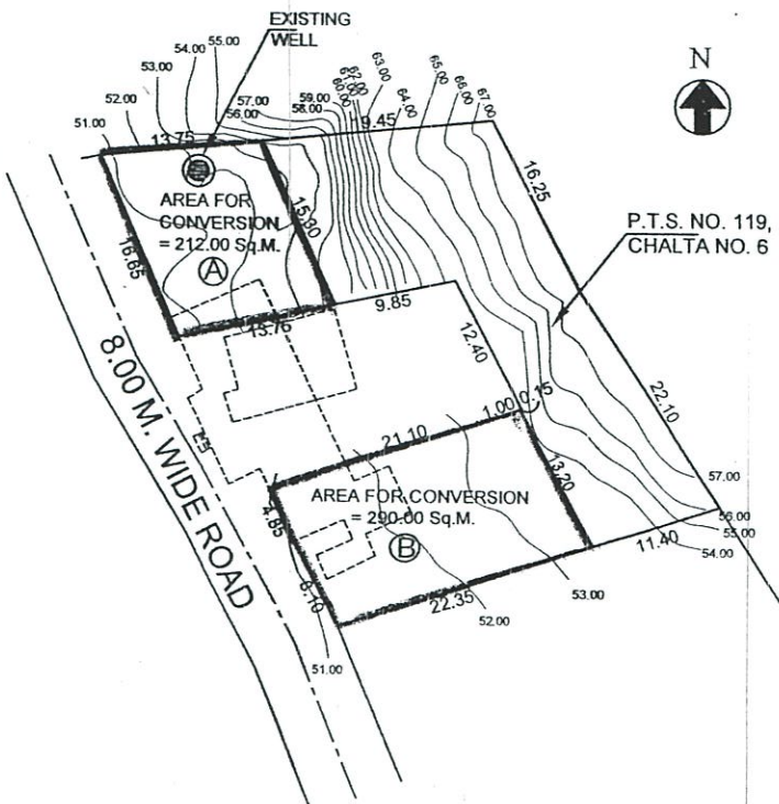
CONTOUR PLAN OF 1M. INTERVAL SCALE:1:500
