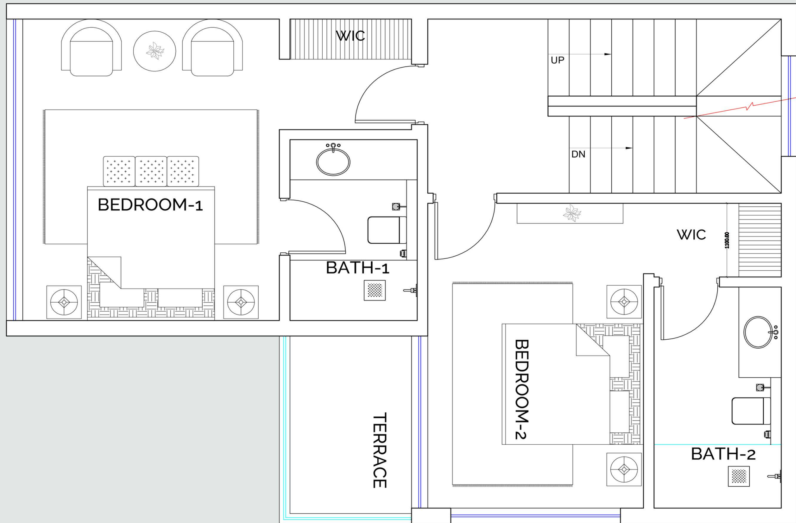
FIRST FLOOR TYPE -02
