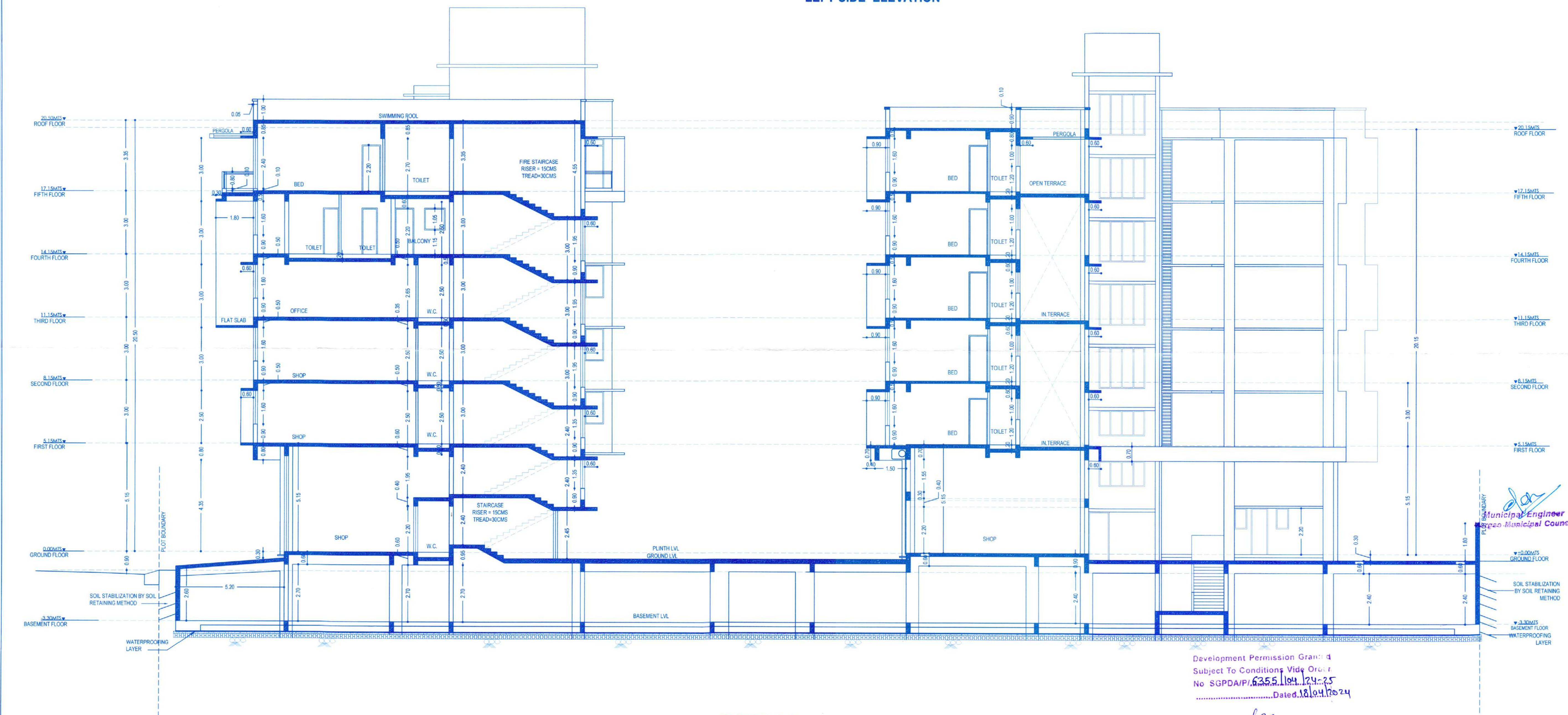
SECTION G-G
