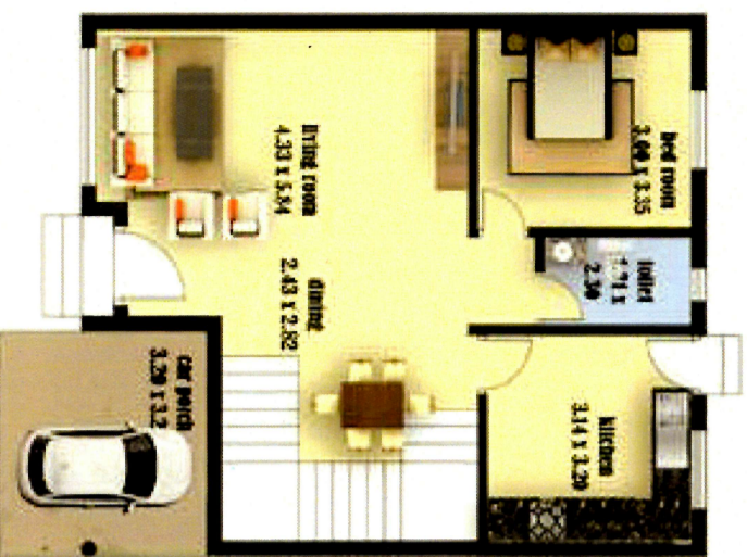
Typical Ground floor plan
