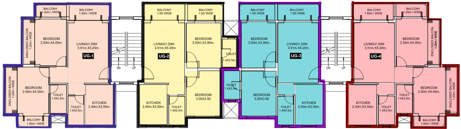
TYPICAL FLOOR PLAN UPPER GROUND
