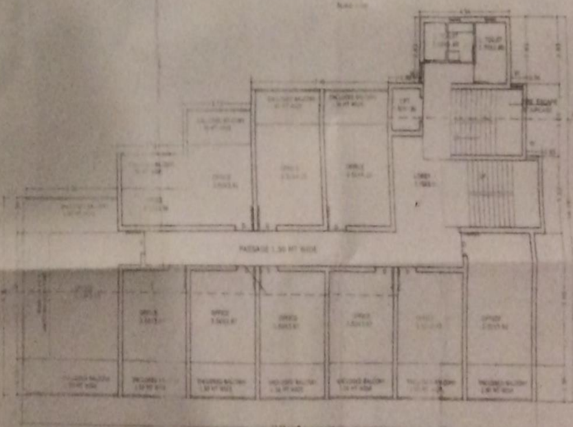
TYPICAL FIRST, SECOND, THIRD, FOURTH, FIFTH & SIXTH FLOOR PLAN
